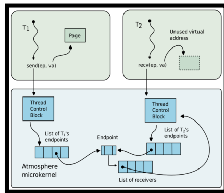
Microkernel
