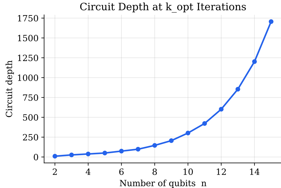
Figure 4 — Circuit Depth & Gate Count
