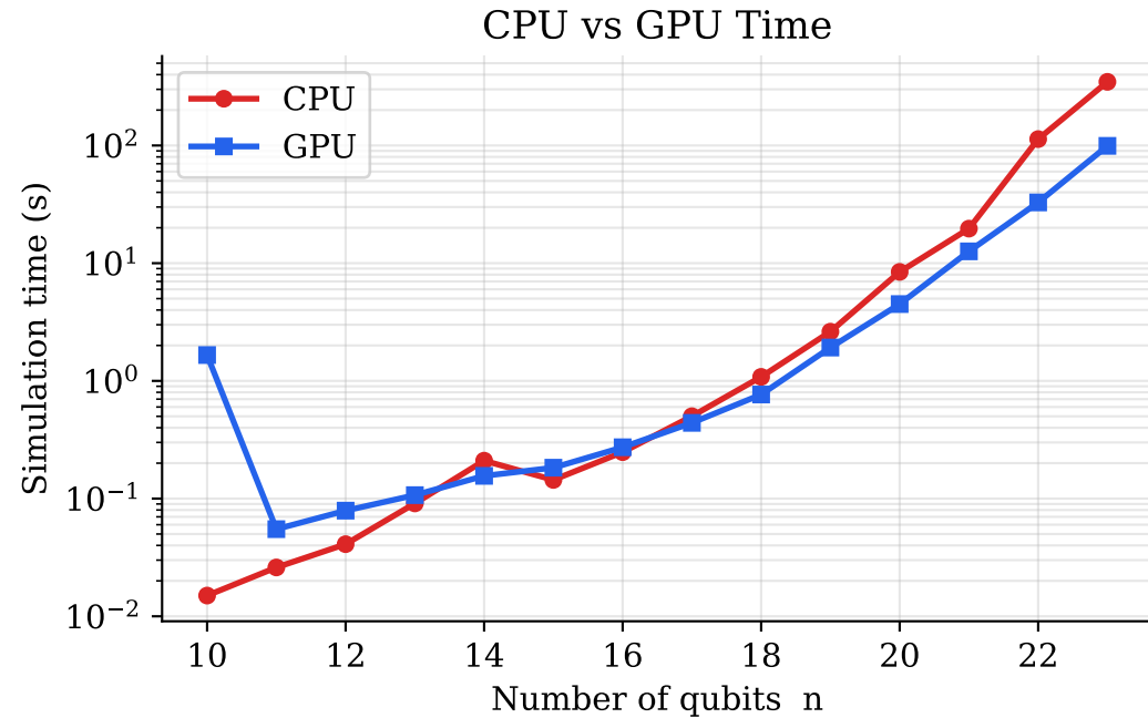
Figure 5 — CPU vs GPU Simulation Time
