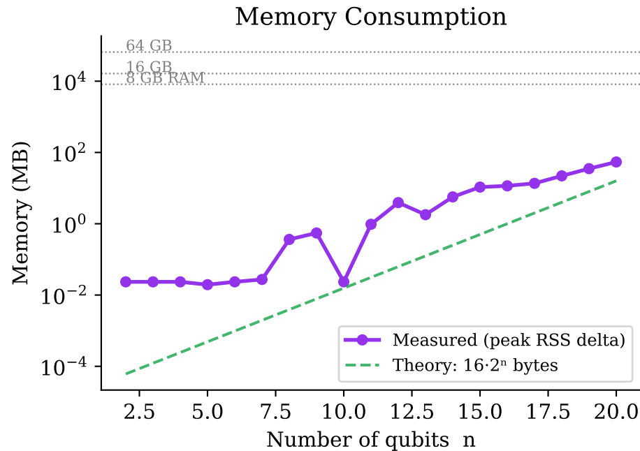
Figure 1 — Classical Simulation Scalability
