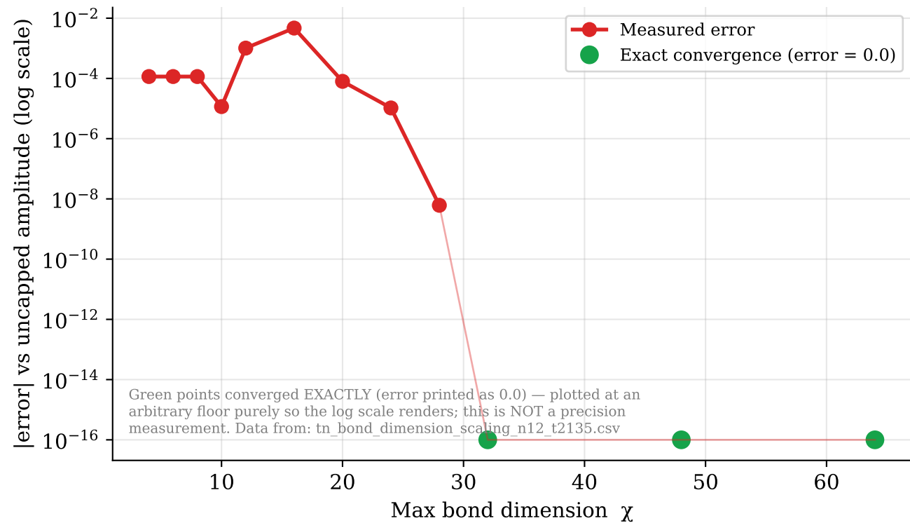
Figure 9 — Convergence vs Bond Dimension (n=12)
