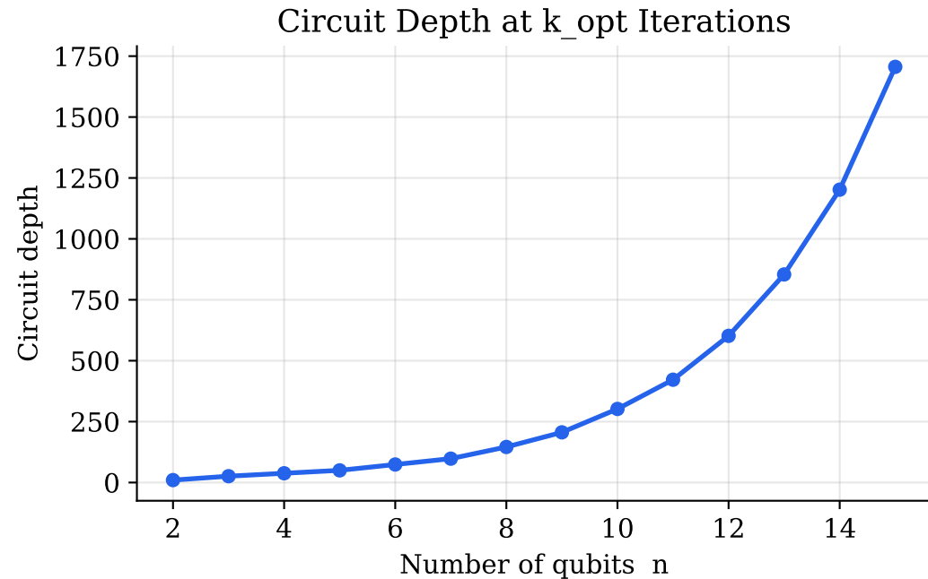
Figure 4 — Circuit Depth & Gate Count
