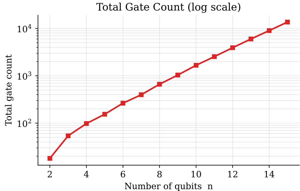
Figure 4 — Circuit Depth & Gate Count
