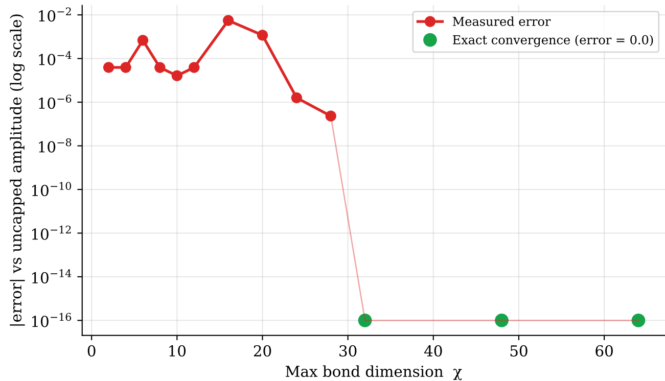
Figure 9 — Convergence vs Bond Dimension (n=11)
