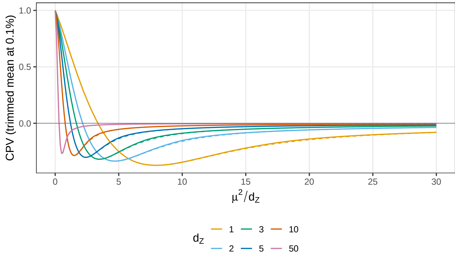
JIVE: Simulated (solid) vs Analytical CPV (dashed)
