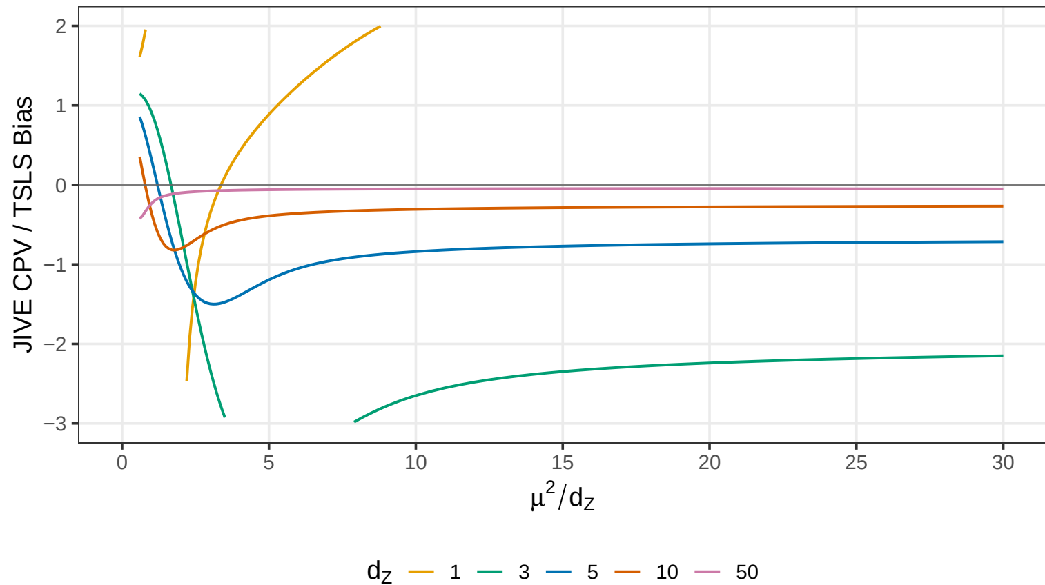
Bias ratio: JIVE overcorrection relative to TSLS
