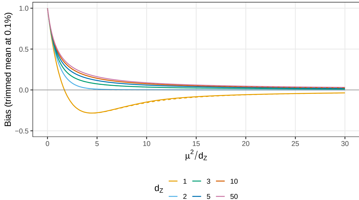
TSLS: Simulated (solid) vs Analytical (dashed)
