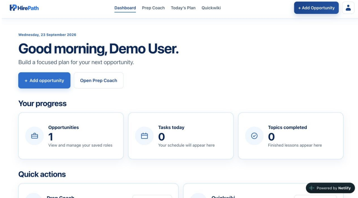
Figure 1 HirePath dashboard
