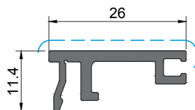
OR 08 Capa Cover | Capot
