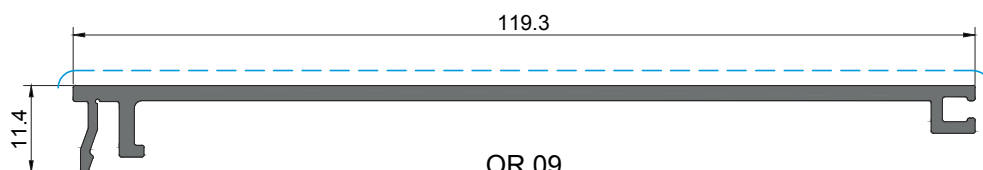
OR 09 Capa Cover | Capot
