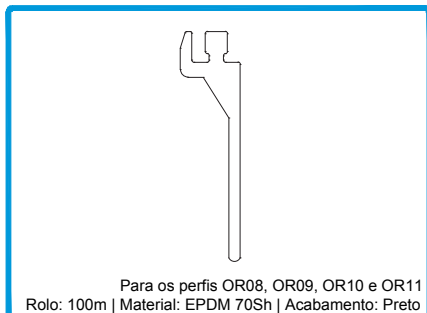
208021 JUNTA VD 1000 GASKET JOINT
