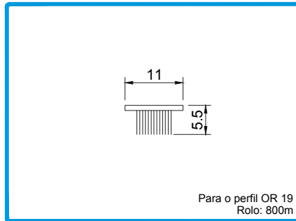
208471 PELÚCIA 11x5.5 CINZA PILE SEAL JOINT BROSSE
