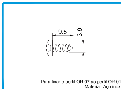
290054 PF DIN7981 3.9x9.5 A2 SCREW VIS
