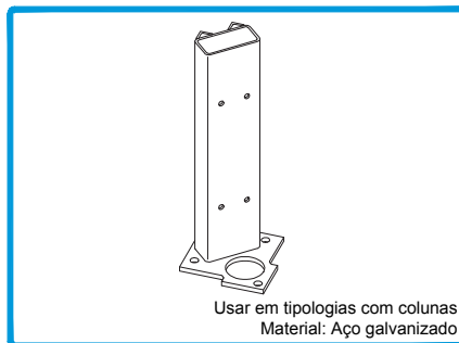
299306 SAPATA SIMPLES SIMPLE ANCHORING ANCRAGE SIMPLE
