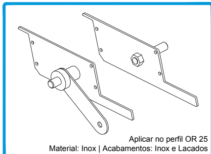
212155 CONJ. TOPOS P/ LAM. MOV. OR25 INOX BRUTO STAINLESS STEEL END CAP KIT KIT D'EMBOUT EN ACIER INOXIDABLE
