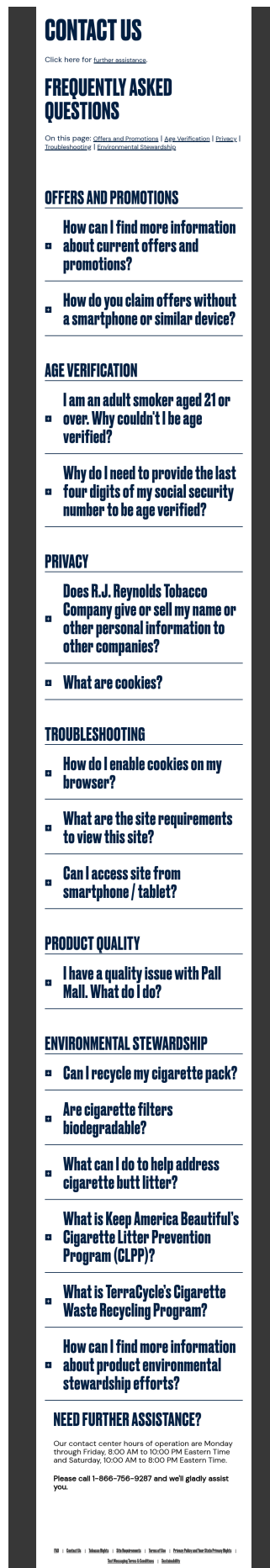
Figure 10: FAQ Template
