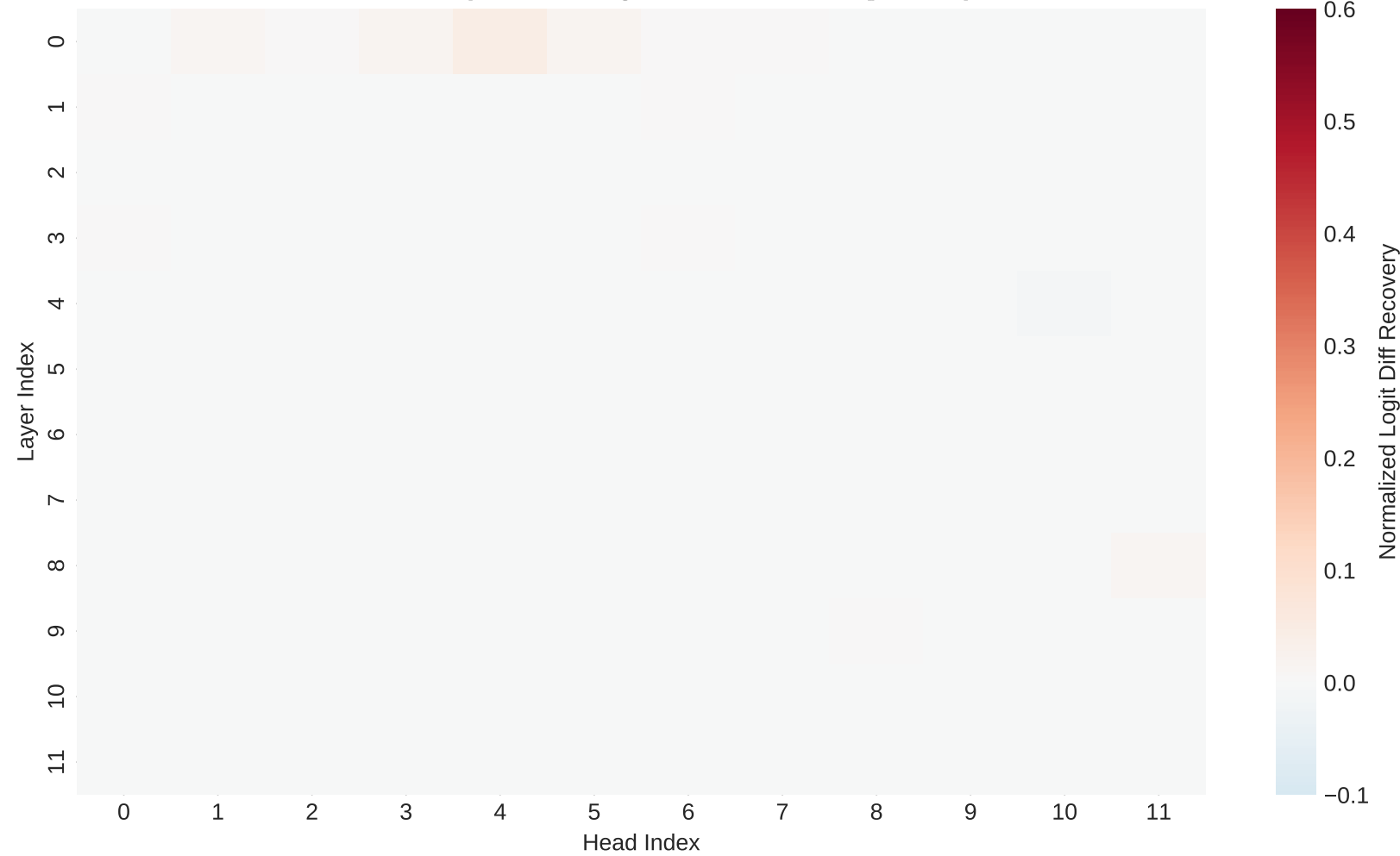
C. Head Output Patching at Final Position ( p = -1 )
