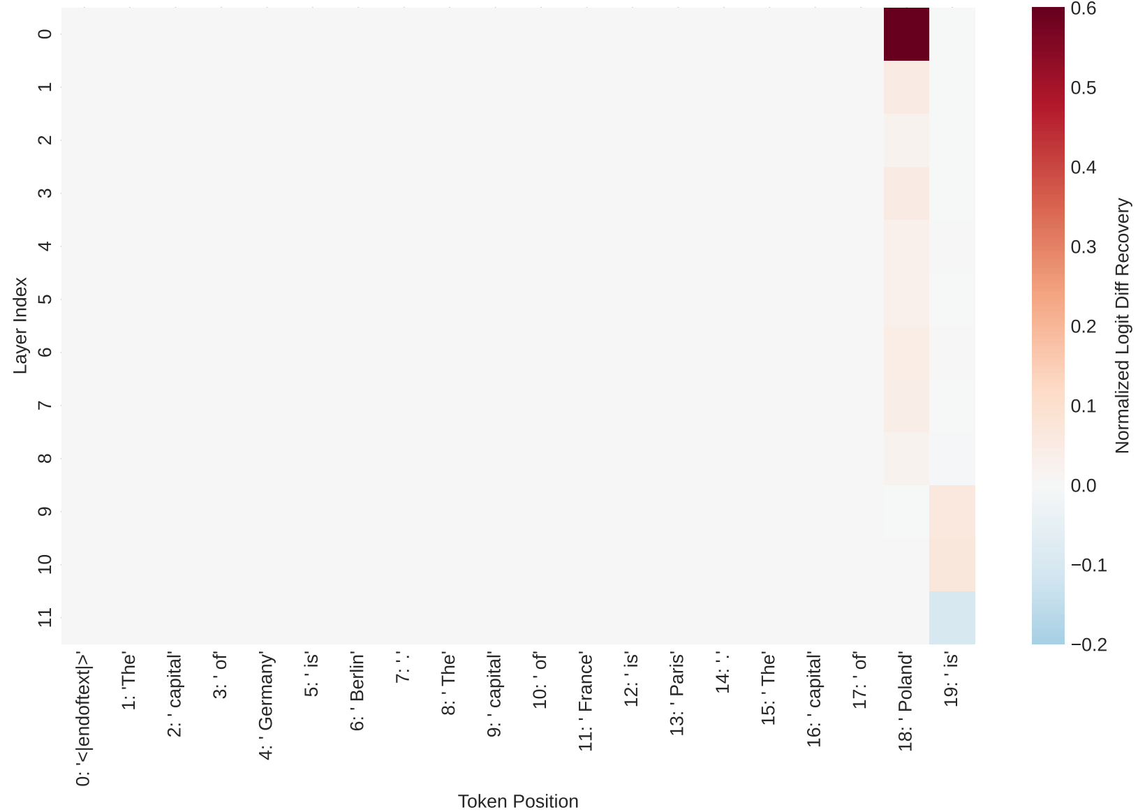
D. Head Output Patching at Subject Position ( p = \text{Subj} )
