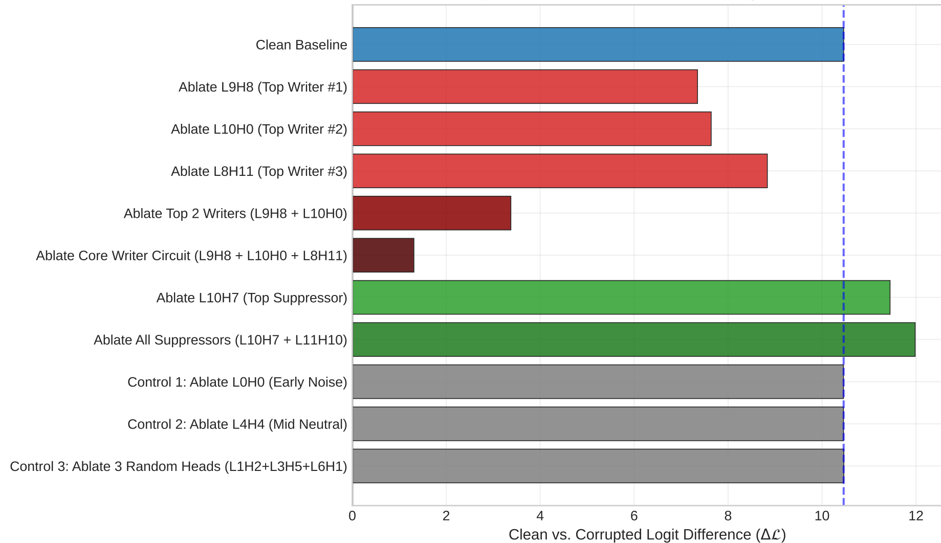
A. Impact of Head Mean-Ablation on Logit Difference
