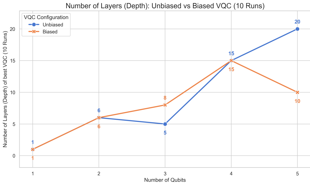
Figure 4.3: Circuit depth in respect to the number of qubits for biased and unbiased classifiers
