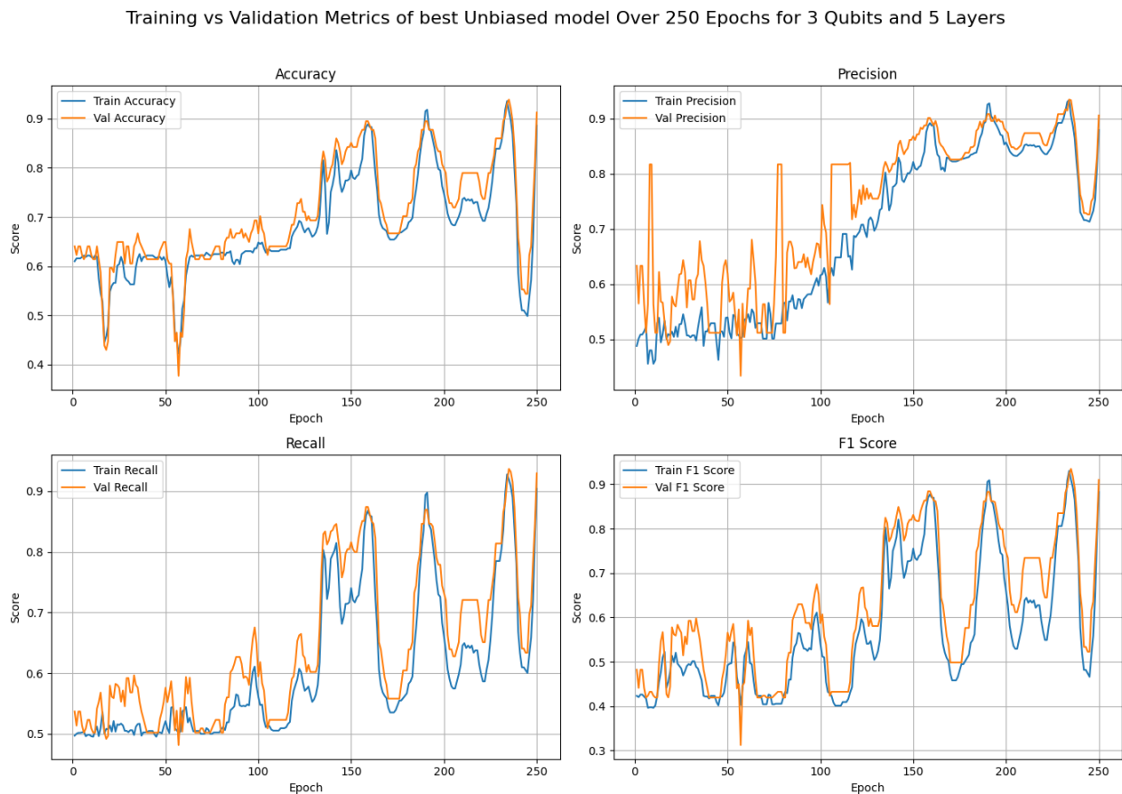
Figure 3.31: Validation and Training curves for the 4 key metrics of the best 3-qubit unbiased classifier
