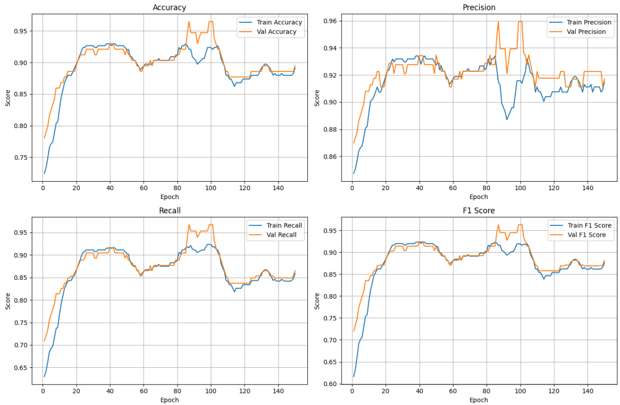
Figure 3.12: Validation and Training curves for the 4 key metrics of the best unbiased 1-qubit VQC
