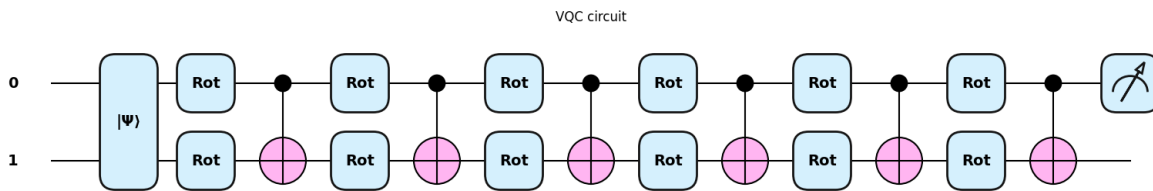
Figure 3.21: Circuit of the best 2-qubit biased classifier
