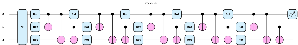
Figure 3.29: Circuit of the best 3-qubit unbiased classifier
