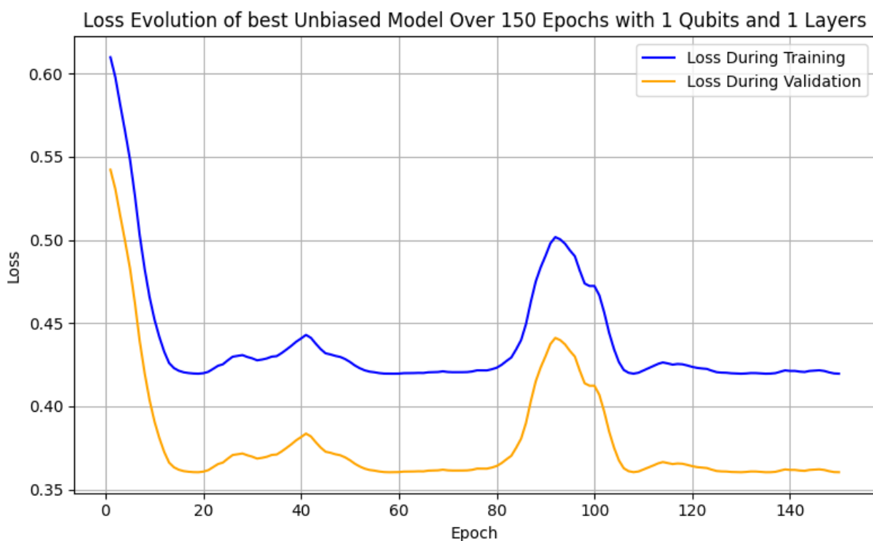
Figure 3.11: Evolution of the loss function of the best unbiased 1-qubit VQC
