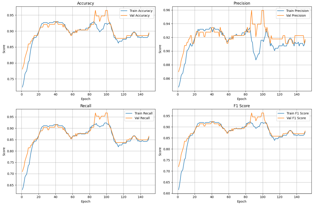
Figure 3.12: Validation and Training curves for the 4 key metrics of the best unbiased 1-qubit VQC
