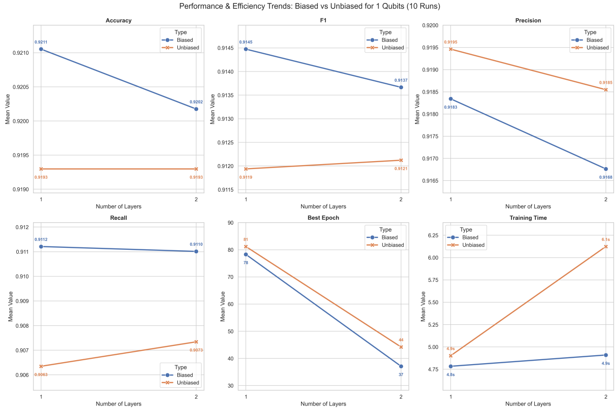
Figure 3.6: Performance and Efficiency Trends of Biased and Unbiased VQC for 1-Qubit
