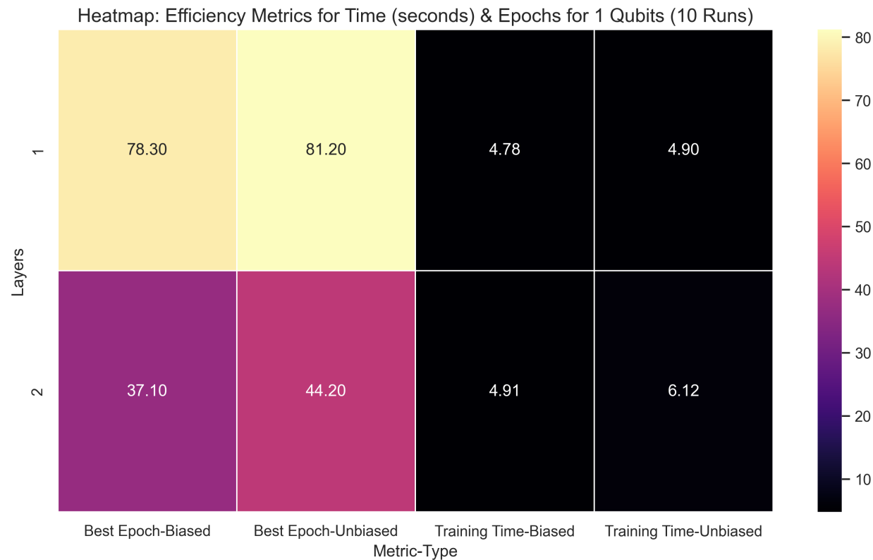
Figure 3.5: Efficiency Results for 1-qubit VQCs after 10 runs
