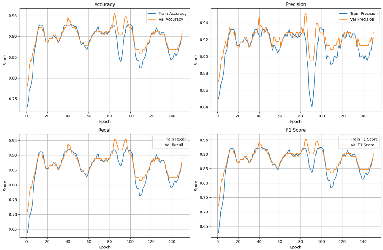
Figure 3.9: Validation and Training curves for the 4 key metrics of the best biased 1-qubit VQC
