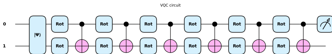
Figure 3.18: Circuit of the best 2-qubit unbiased classifier
