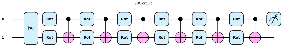
Figure 3.1: A VQC's circuit configuration comprising of two qubits and six layers
