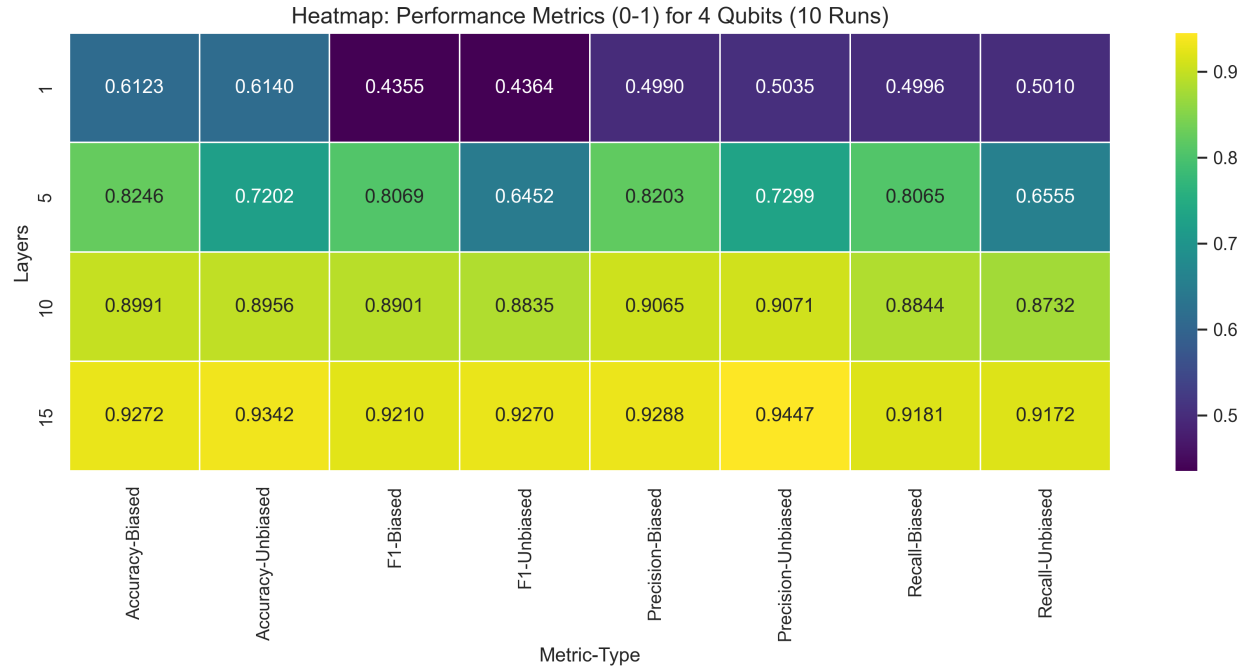
Figure 3.37: Performance Results for 4-qubit classifiers after 10 runs
