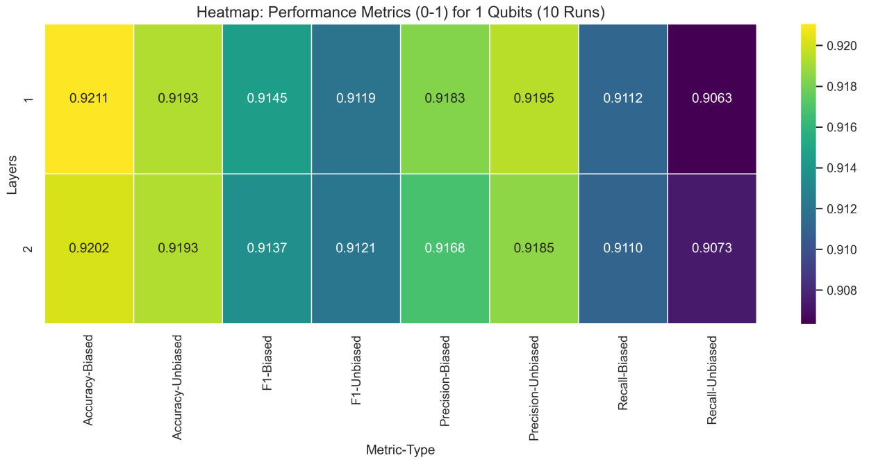
Figure 3.4: Performance Results for 1-qubit VQCs after 10 runs
