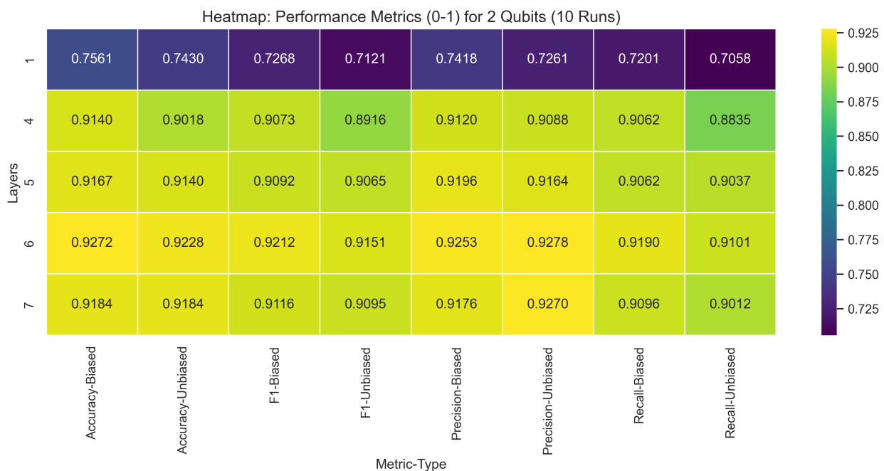
Figure 3.15: Performance Results for 2-qubit VQCs after 10 runs
