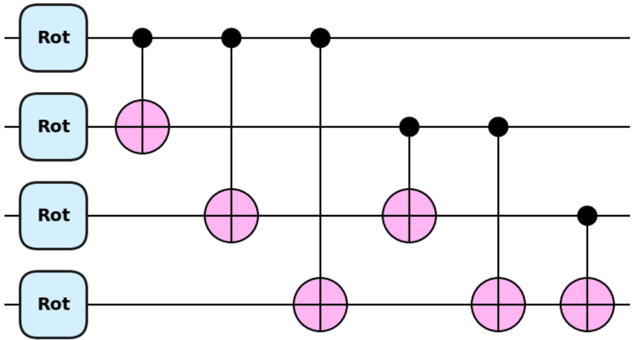
Figure 3.36: A single layer of the 4-qubit VQC circuit
