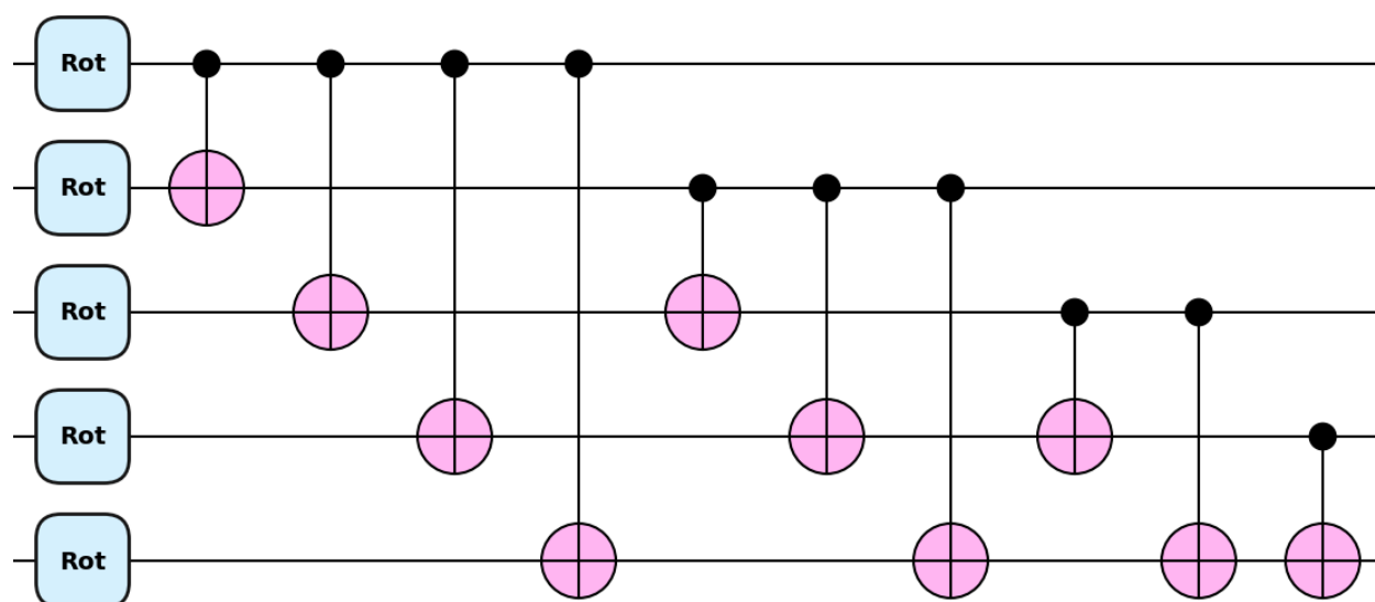
Figure 3.46: A single layer of the 5-qubit VQC circuit
