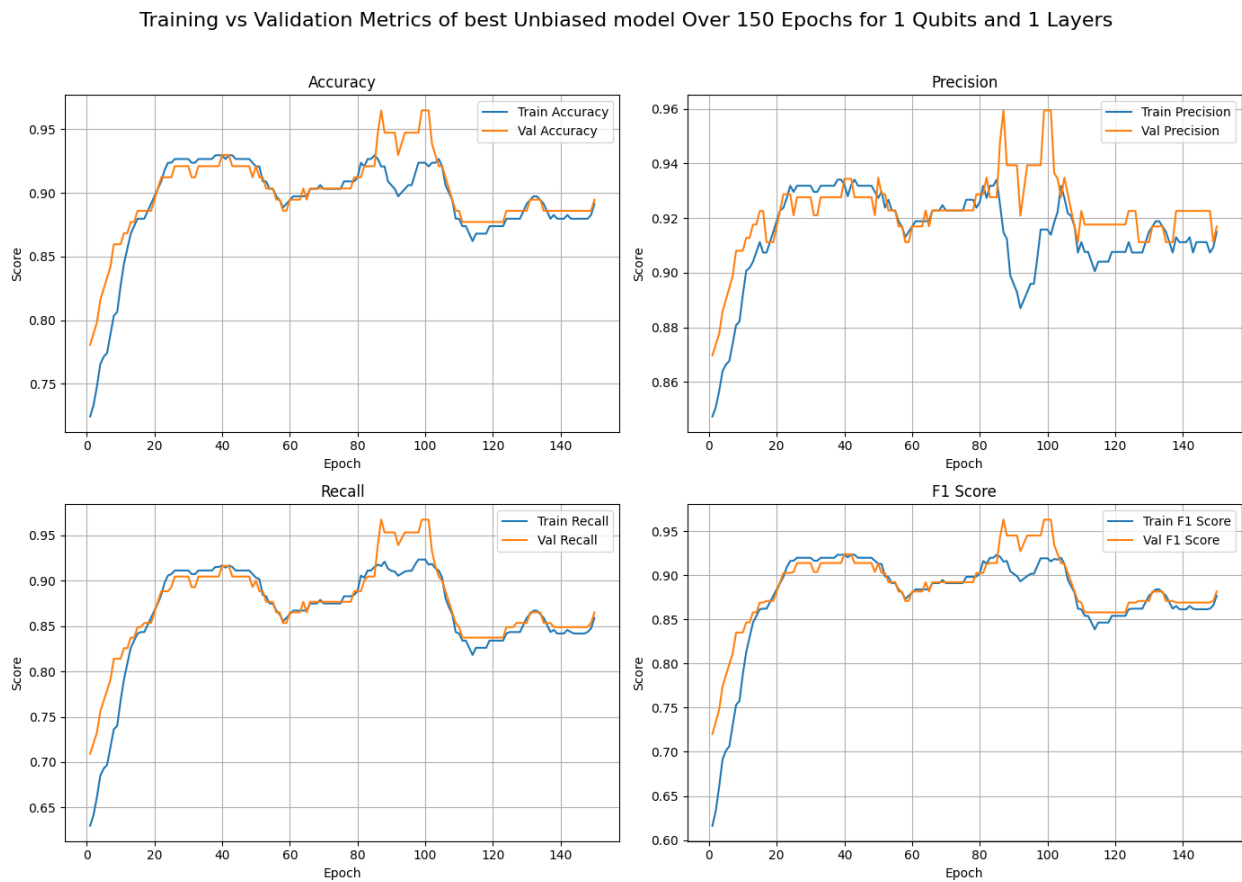
Figure 3.12: Validation and Training curves for the 4 key metrics of the best unbiased 1-qubit VQC
