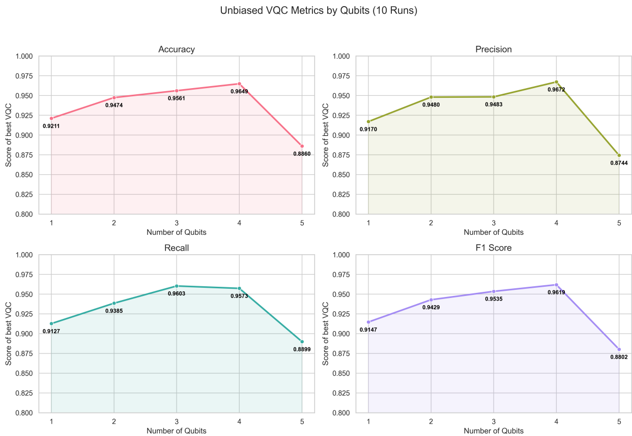
Figure 4.1: Performance of best unbiased classifier per number of qubits across all runs
