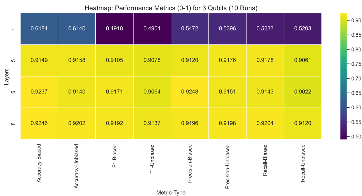
Figure 3.26: Performance Results for 3-qubit classifiers after 10 runs
