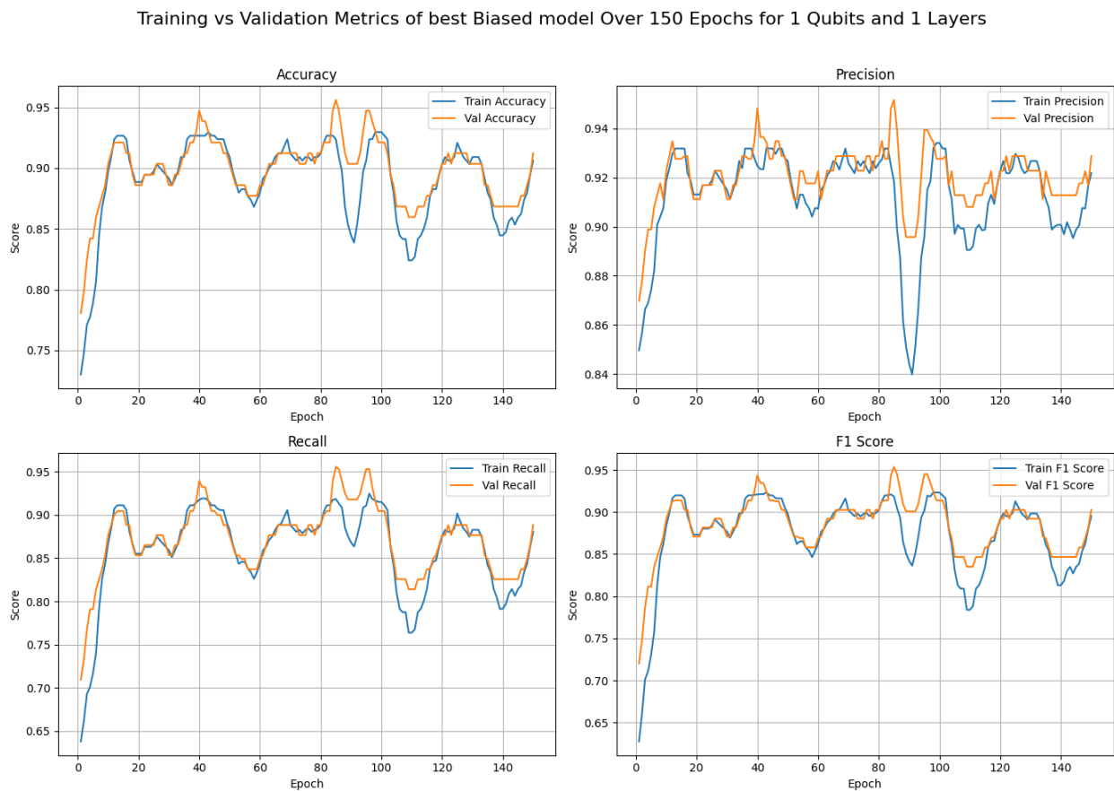
Figure 3.9: Validation and Training curves for the 4 key metrics of the best biased 1-qubit VQC
