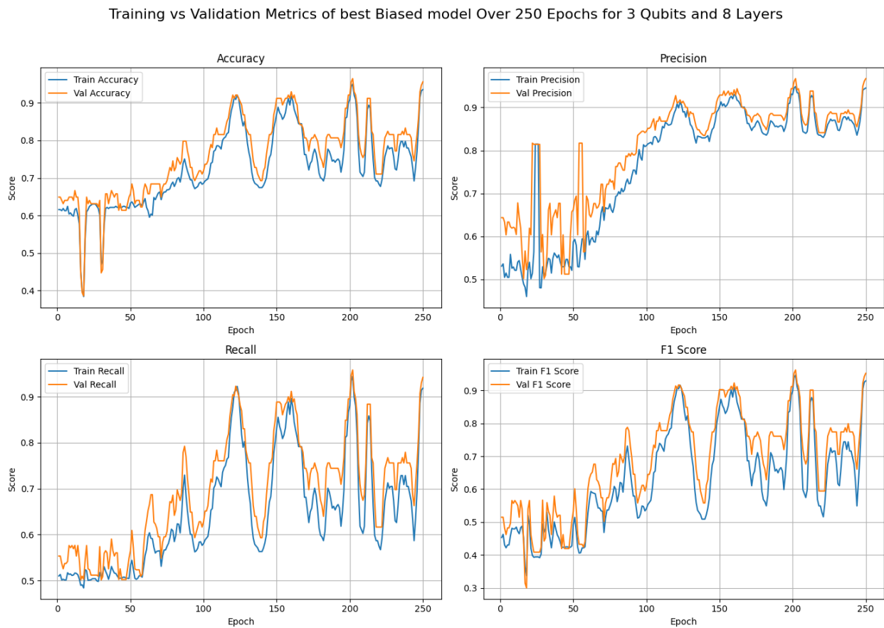
Figure 3.34: Validation and Training curves for the 4 key metrics of the best 3-qubit biased classifier
