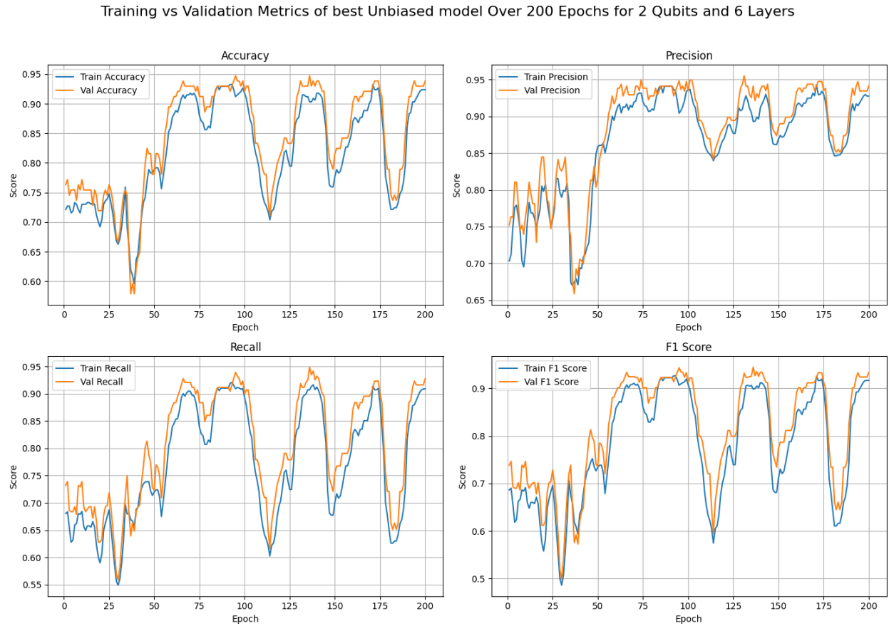
Figure 3.20: Validation and Training curves for the 4 key metrics of the best 2-qubit unbiased classifier
