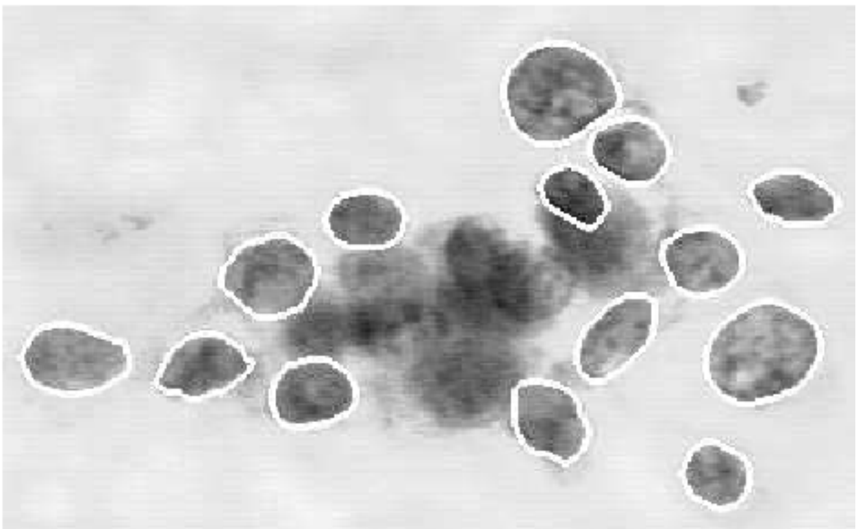
Figure 2.1: A magnified image of a malignant breast FNA with the visible cell nuclei having been outlined with the help of a curve fitting program [3].
