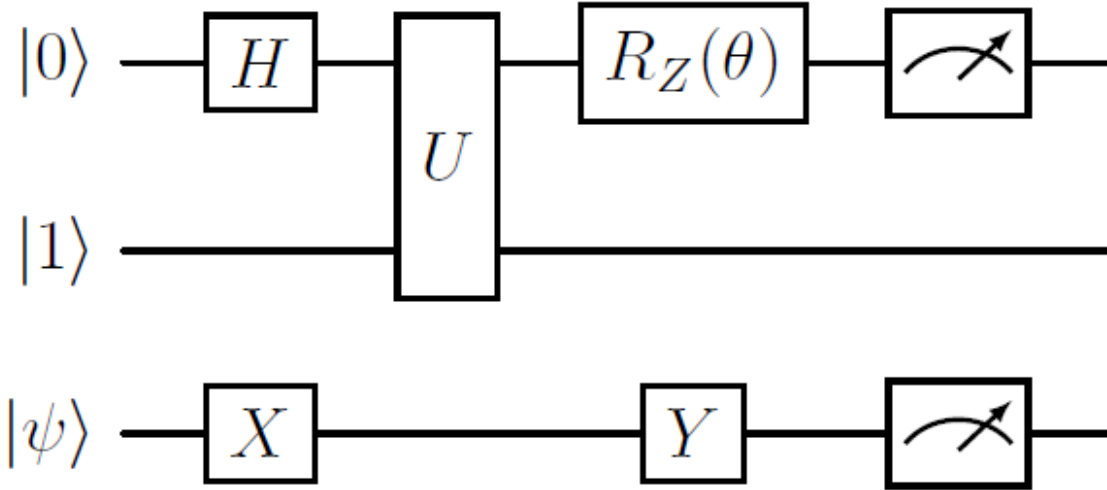
Figure 1.2: An example of a quantum circuit diagram [2]
