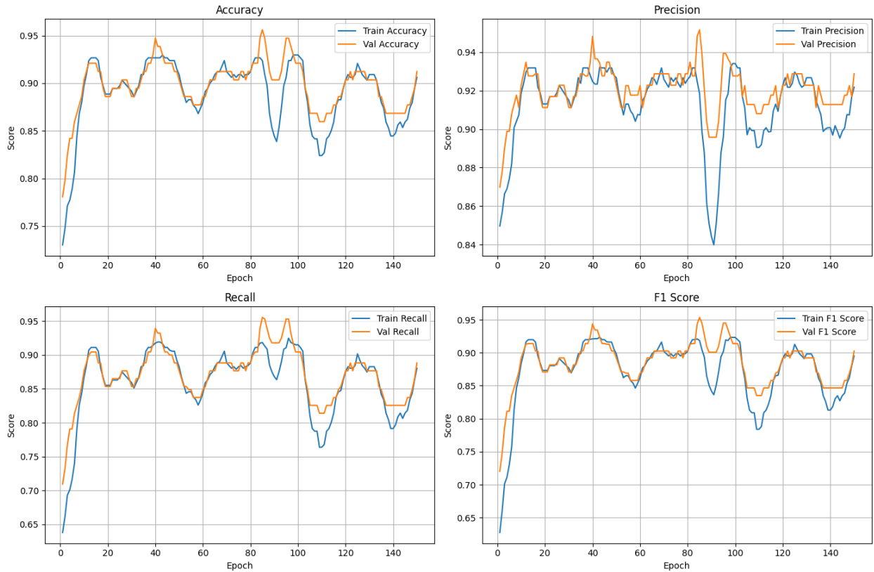
Figure 3.9: Validation and Training curves for the 4 key metrics of the best biased 1-qubit VQC
