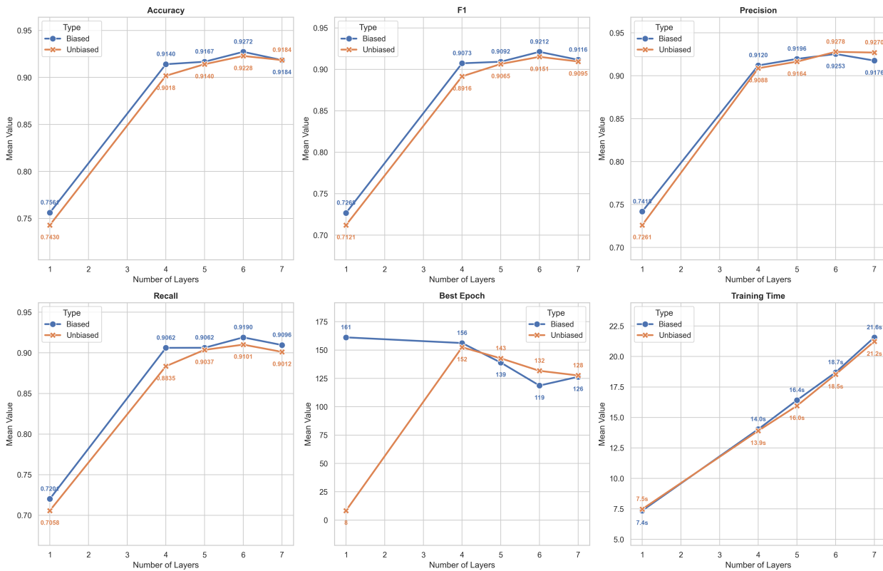
Figure 3.17: Performance and Efficiency Trends of Biased and Unbiased Classifier for 2 Qubits
