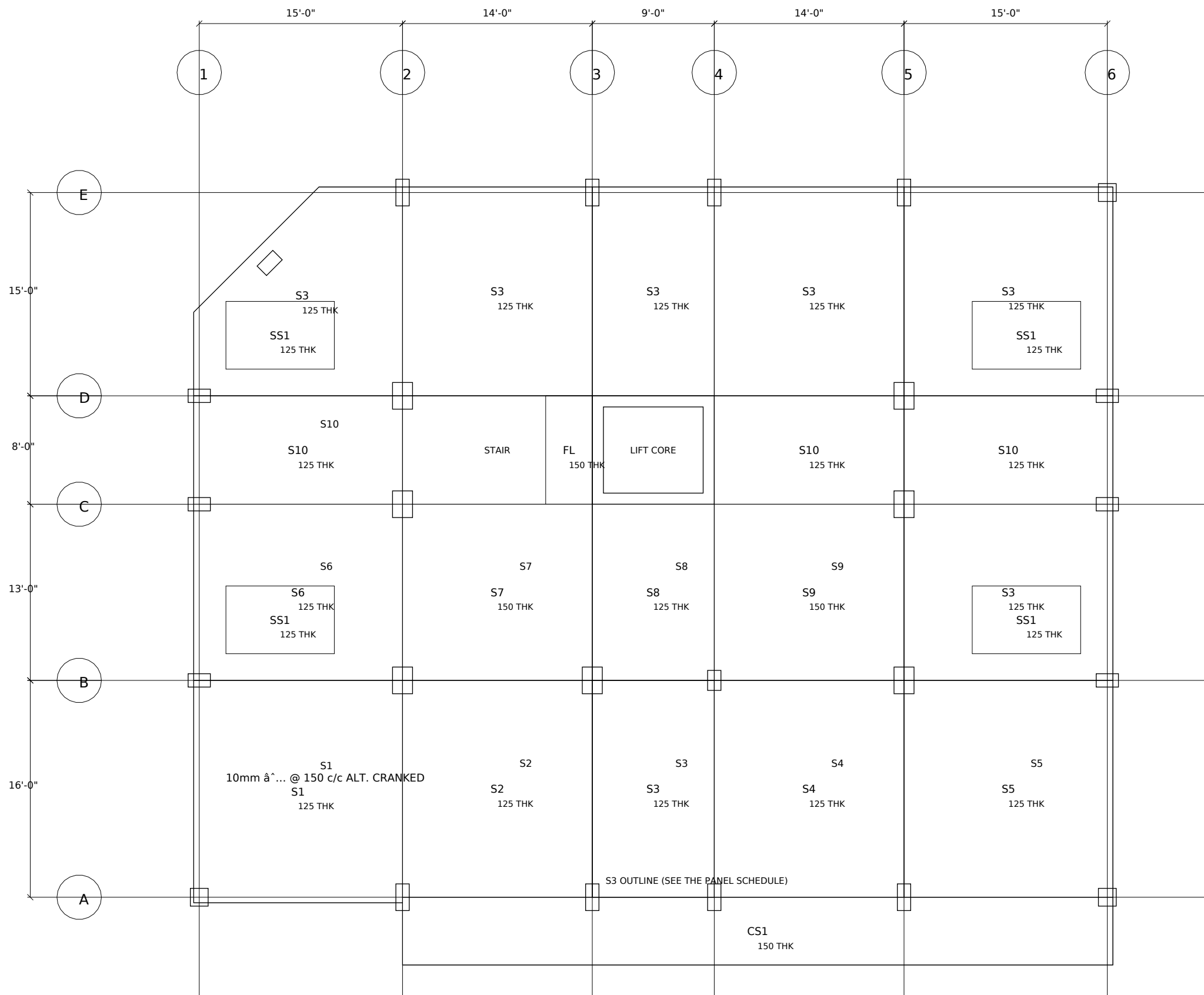
TYPICAL SLAB REINFORCEMENT PLAN
