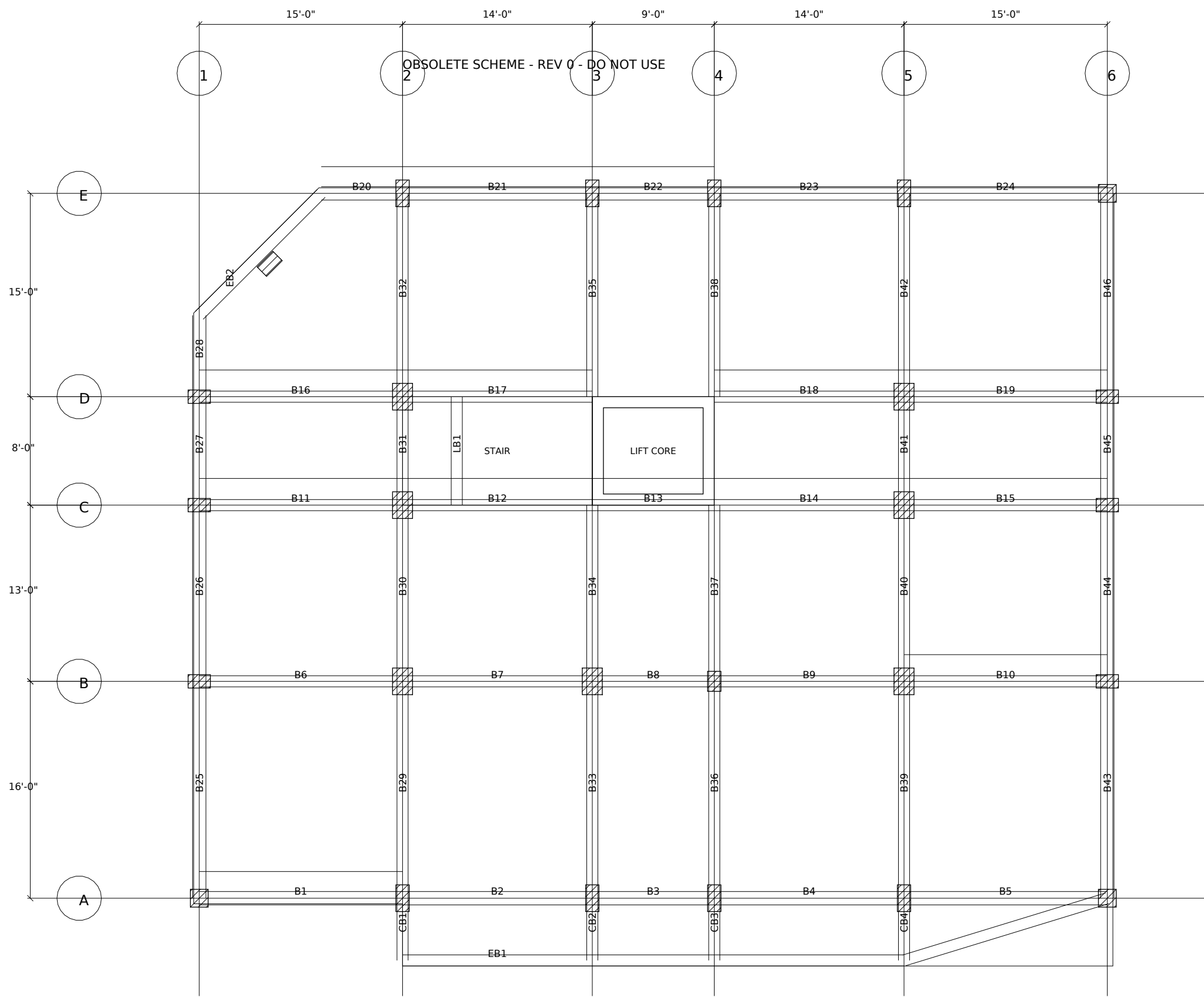
TYPICAL FLOOR BEAM LAYOUT (2ND TO 6TH FLOOR)
