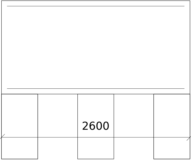
PC4
