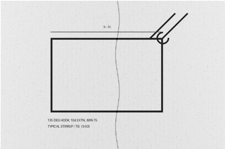
PASTED DETAIL - HOOK (SCANNED FROM THE STANDARD SHEET)
