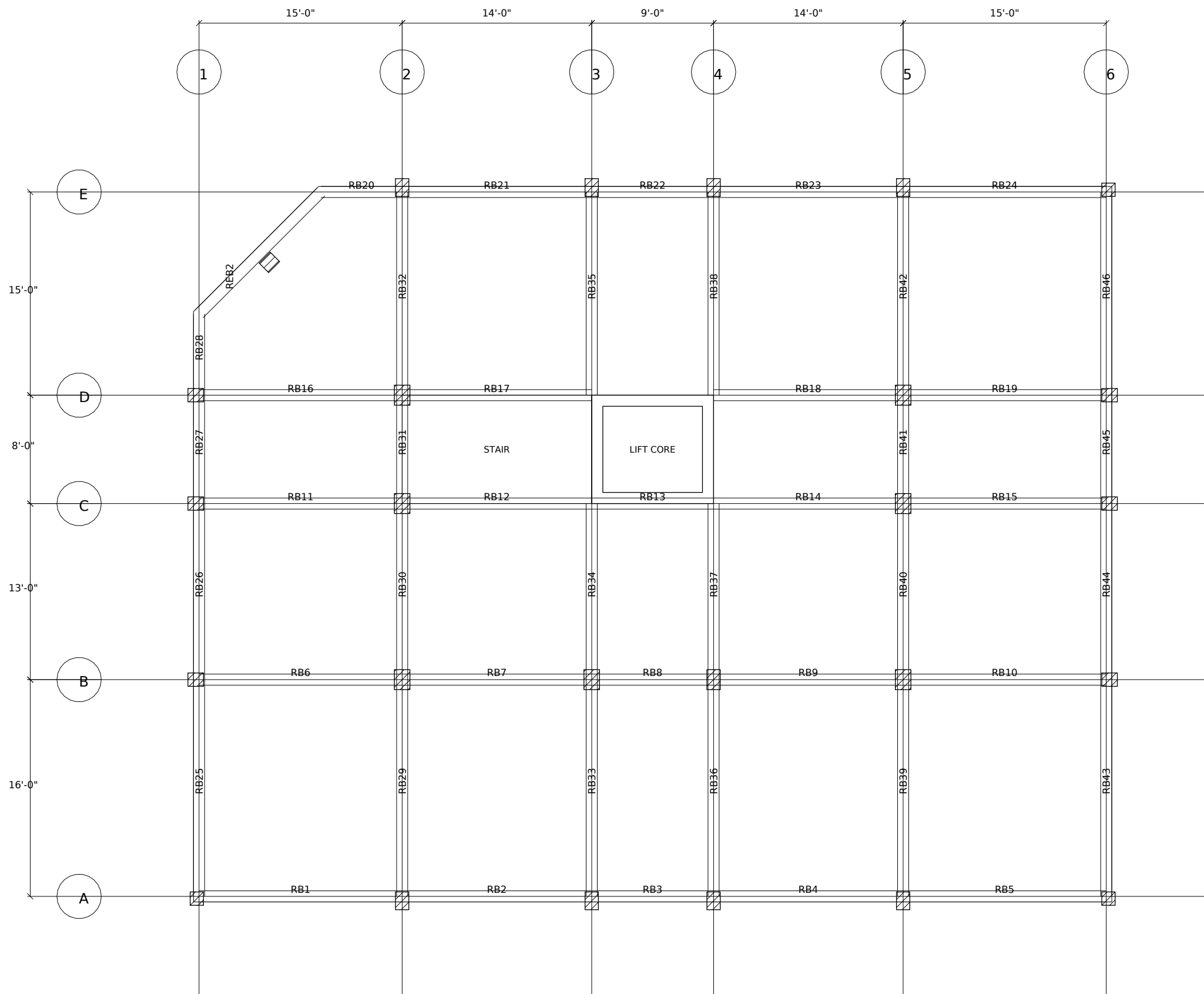
ROOF BEAM LAYOUT (AT ROOF LEVEL)
