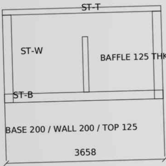
SEPTIC TANK
