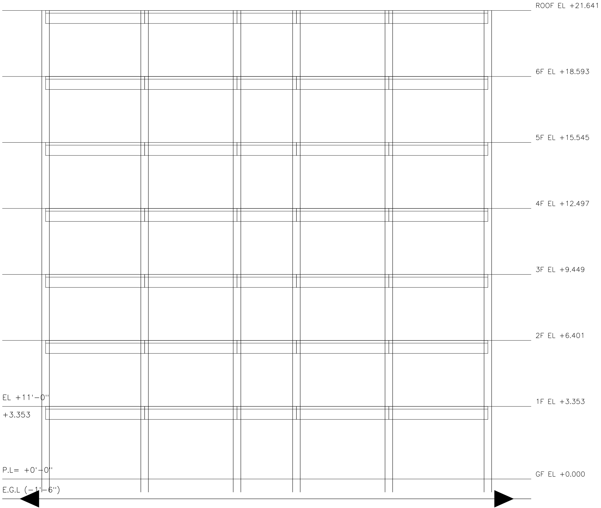
SECTION A–A
