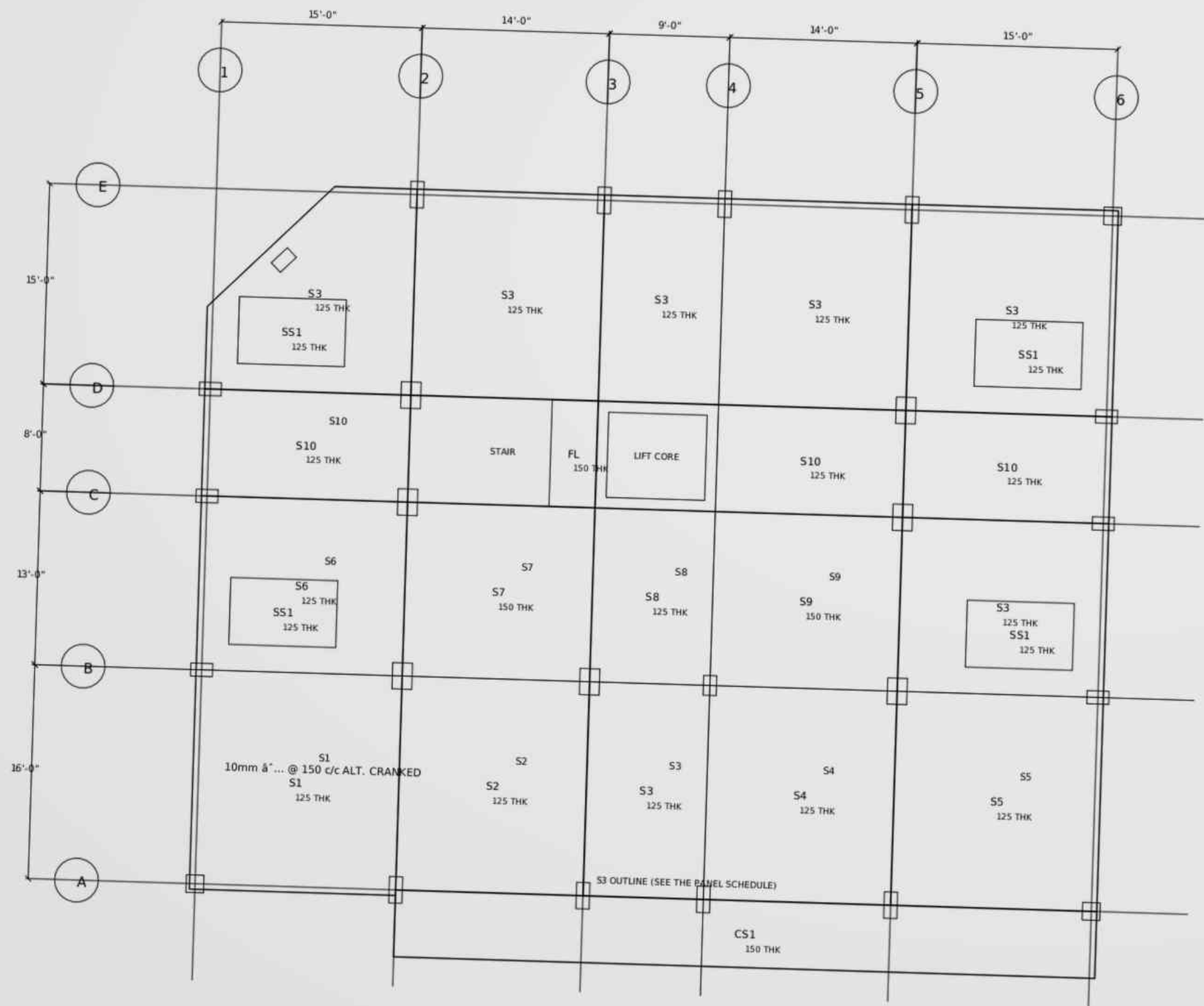
TYPICAL SLAB REINFORCEMENT PLAN
