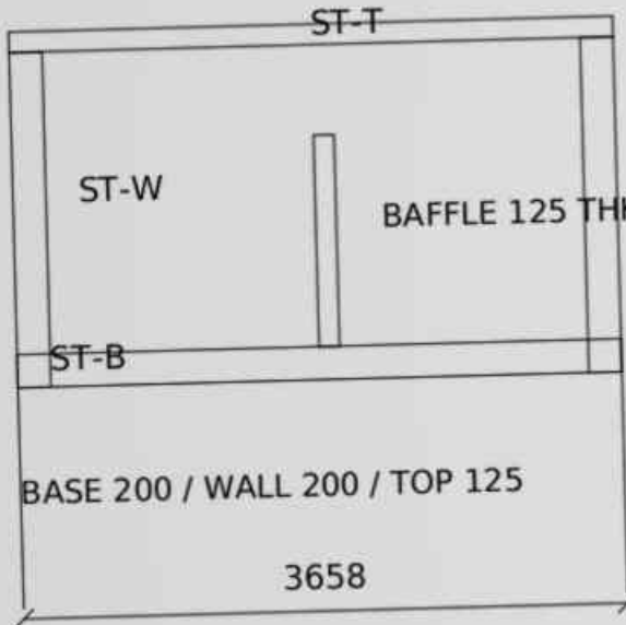
SEPTIC TANK
