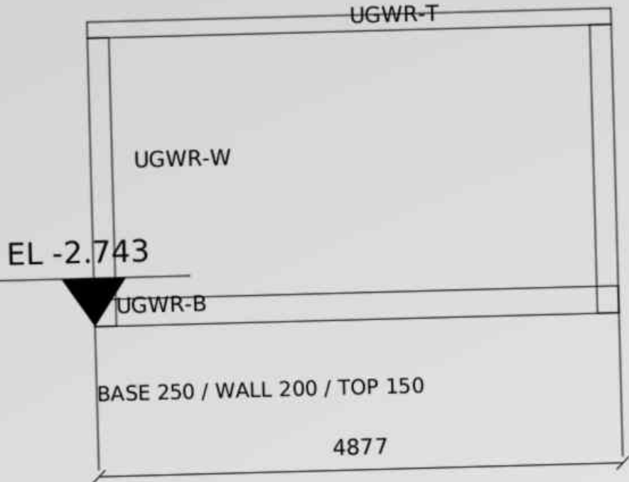
UNDERGROUND WATER RESERVOIR
