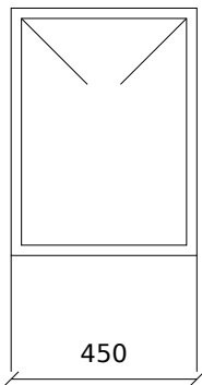
135° HOOK, 10d EXTENSION TYPICAL STIRRUP / TIE 10Ø @ 100 c/c
