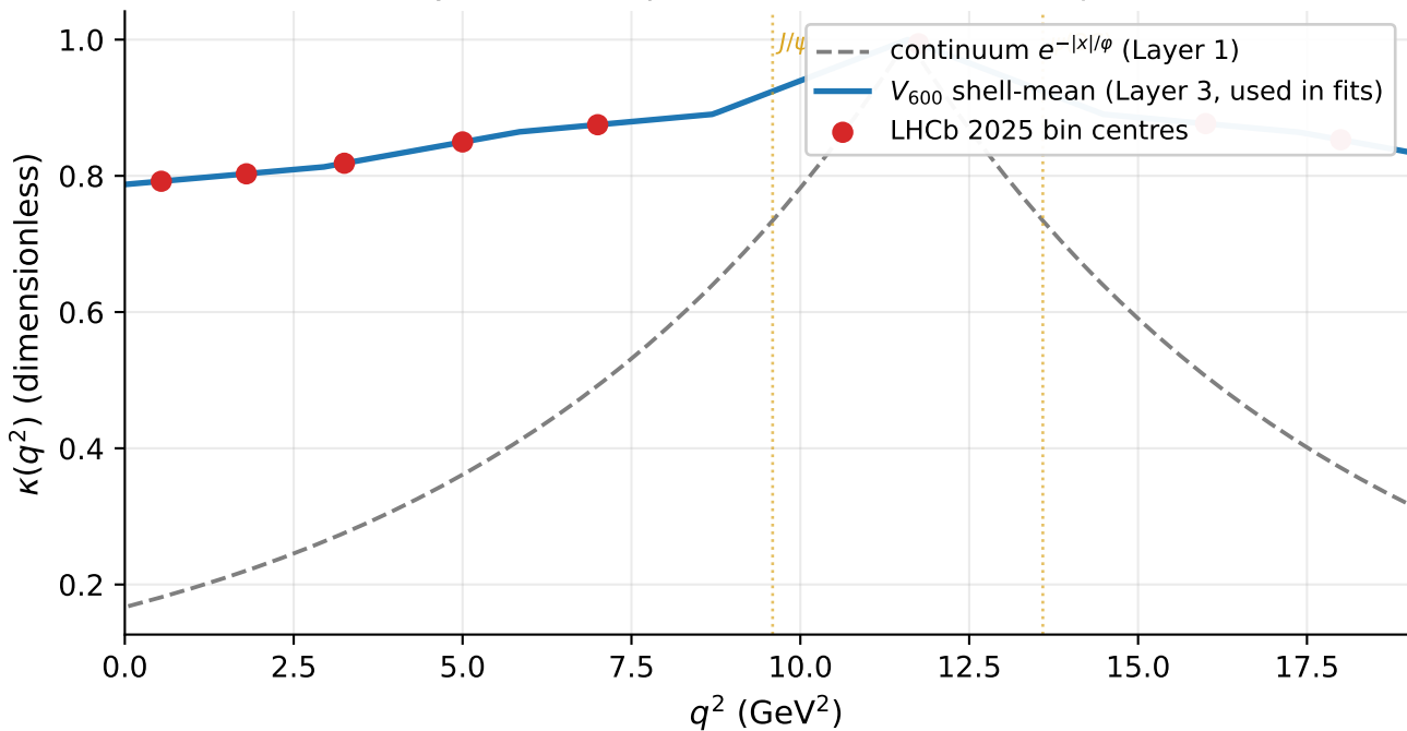
Geometry-derived response kernel on the LHCb q^2 window
