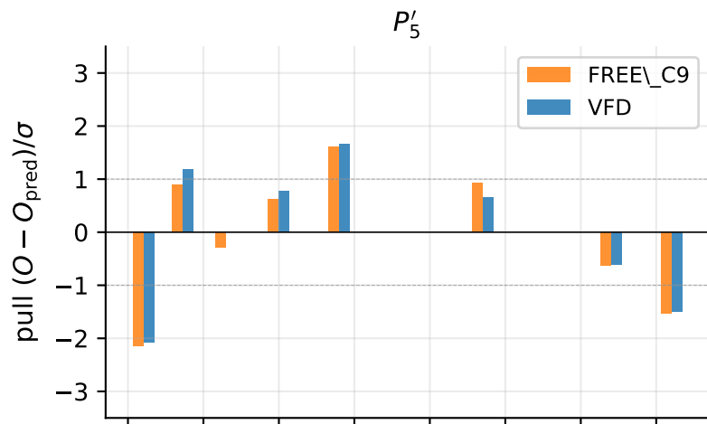
LHCb 2025 bin pulls under non-linear FREE\_C9 and VFD fits (32 bins, 4 obs)
