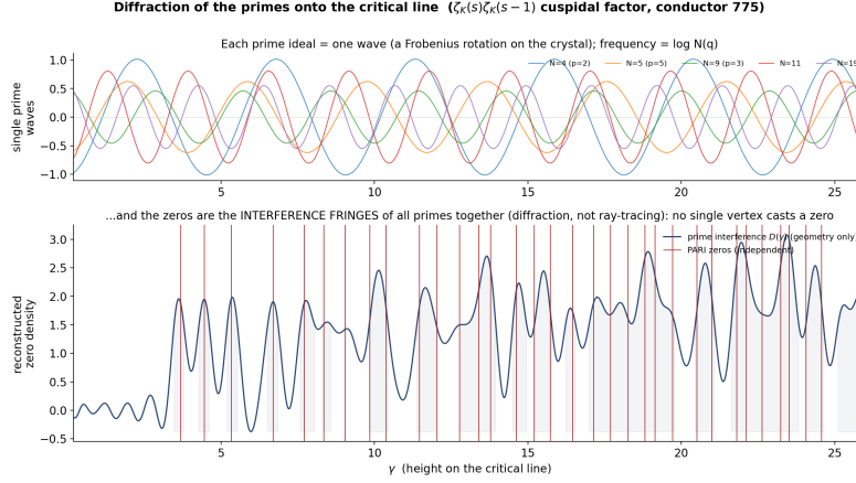
Figure 2: Each prime ideal is a wave (top); their geometry-only interference D(\gamma) has fringes where the independently-computed zeros (red) sit (bottom). The zeros are a collective feature of all the prime-waves: each wave has global support in \gamma , so no single prime determines a zero.
