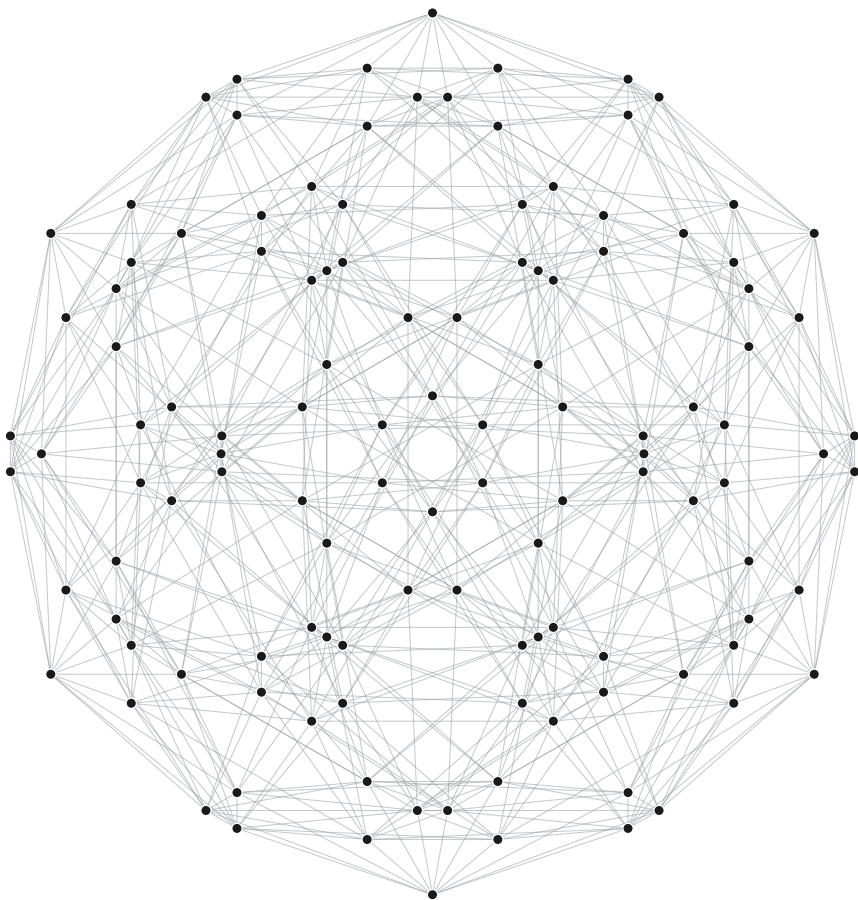
The 600-cell: 120 corners, 720 edges
