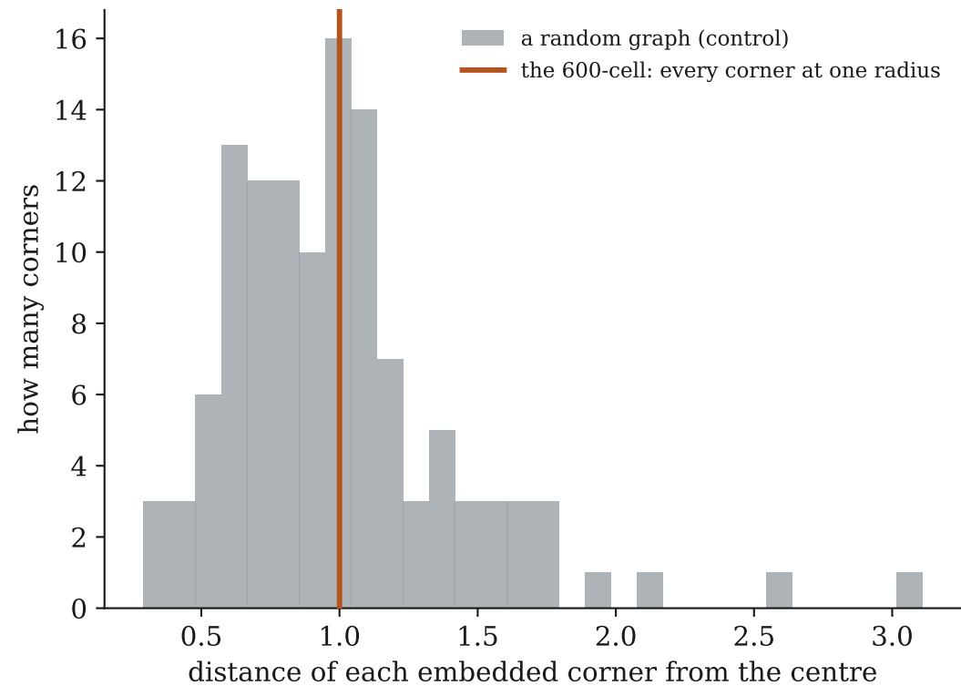
The corners land on a single sphere
