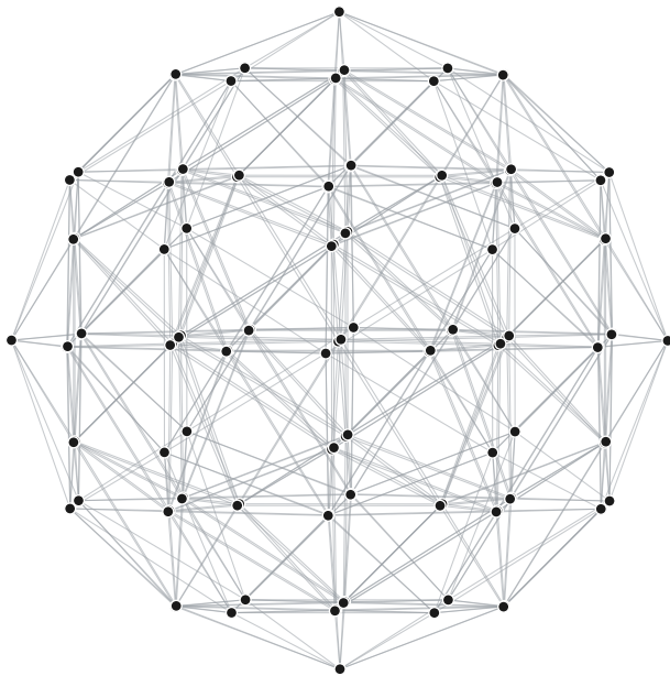
...and rebuild the 600-cell
