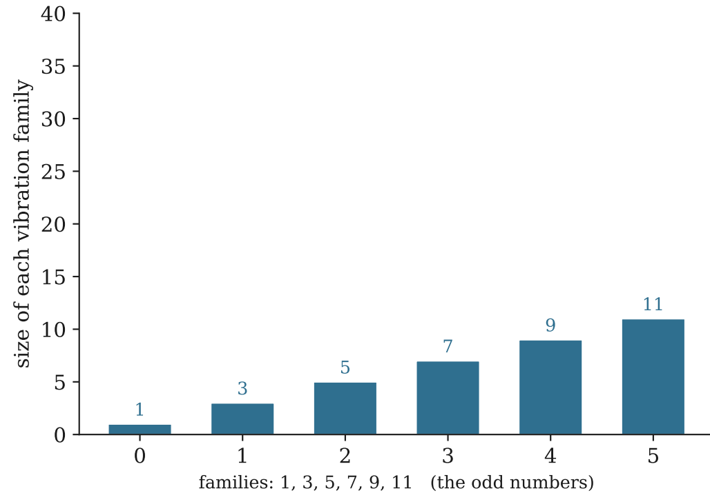
the ordinary 2-sphere
