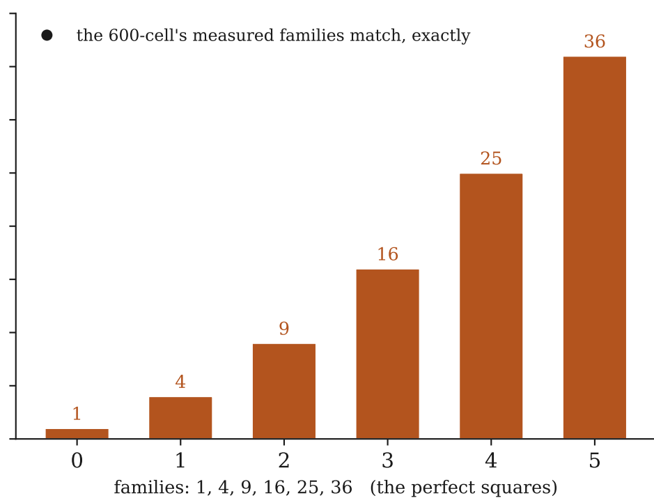
the 3-sphere — and the crystal
