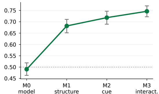
(b) Nested variance partition
