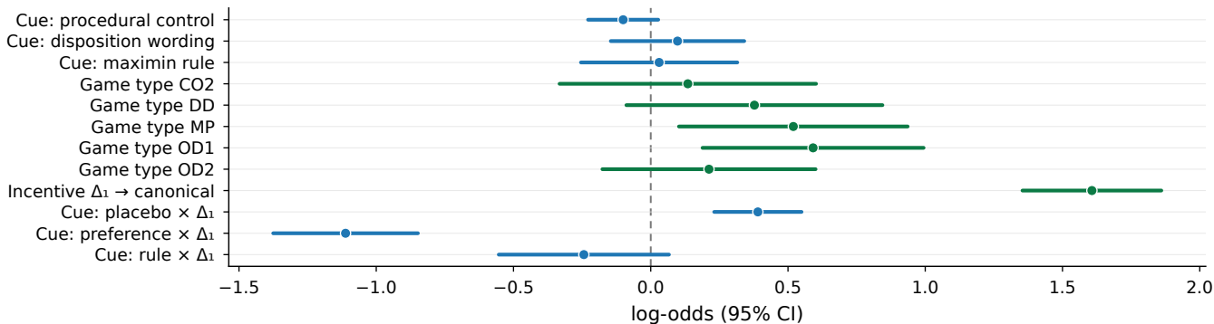
(c) GLMM cross-check
