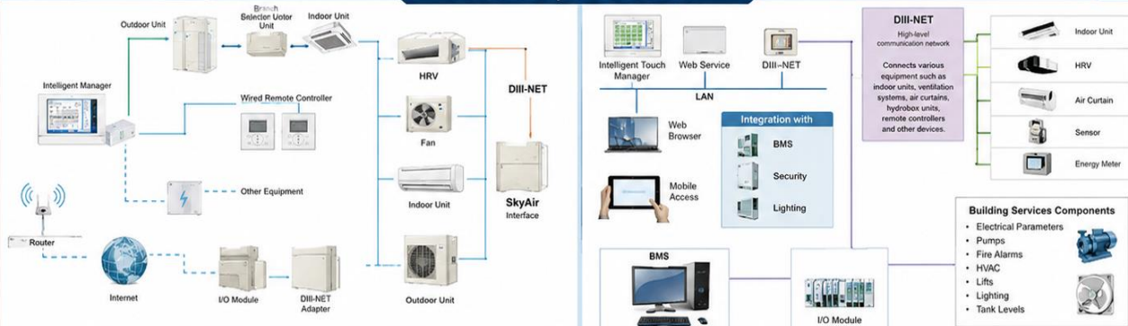
BACnet Gateway
