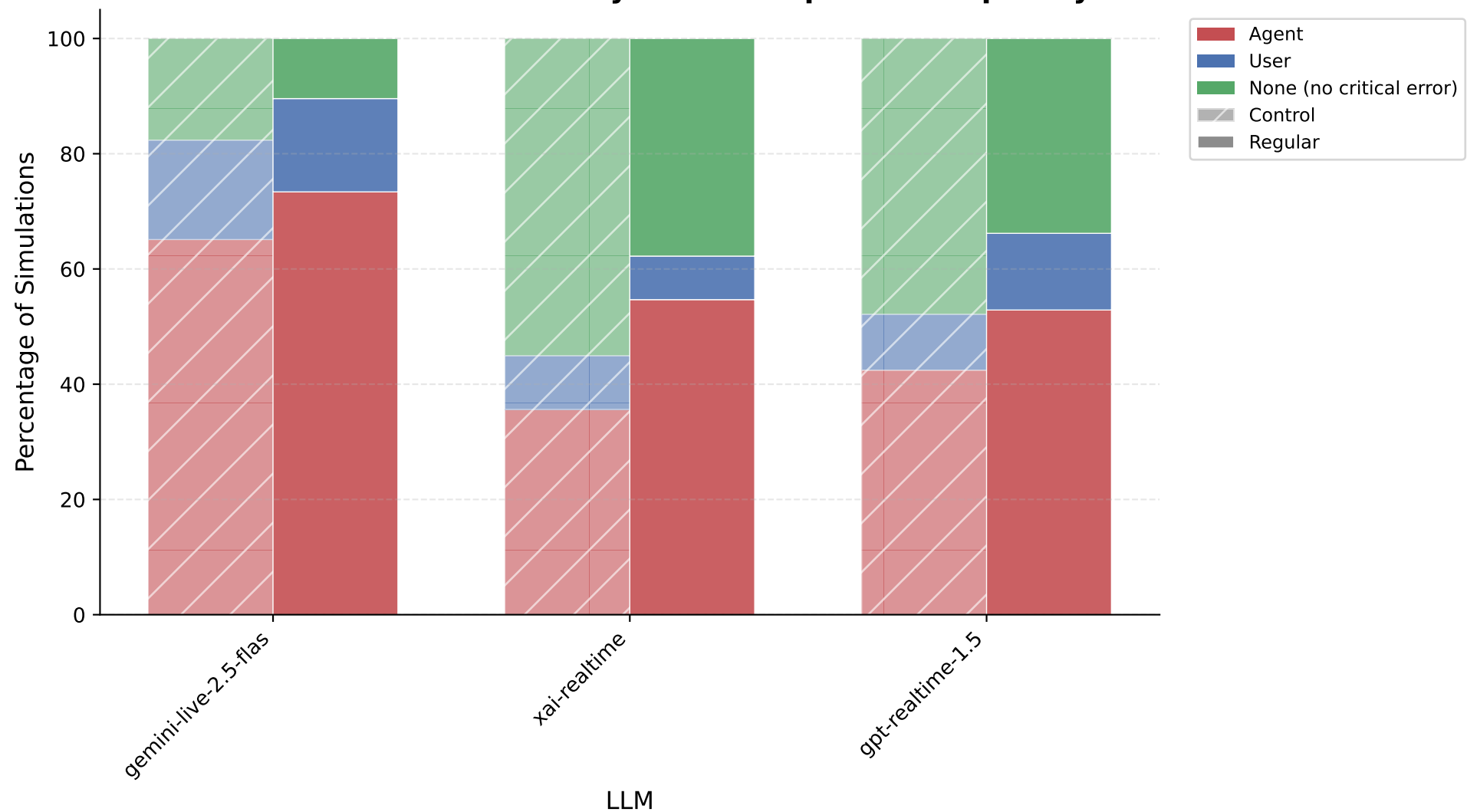
First Critical Error Source by LLM and Speech Complexity
