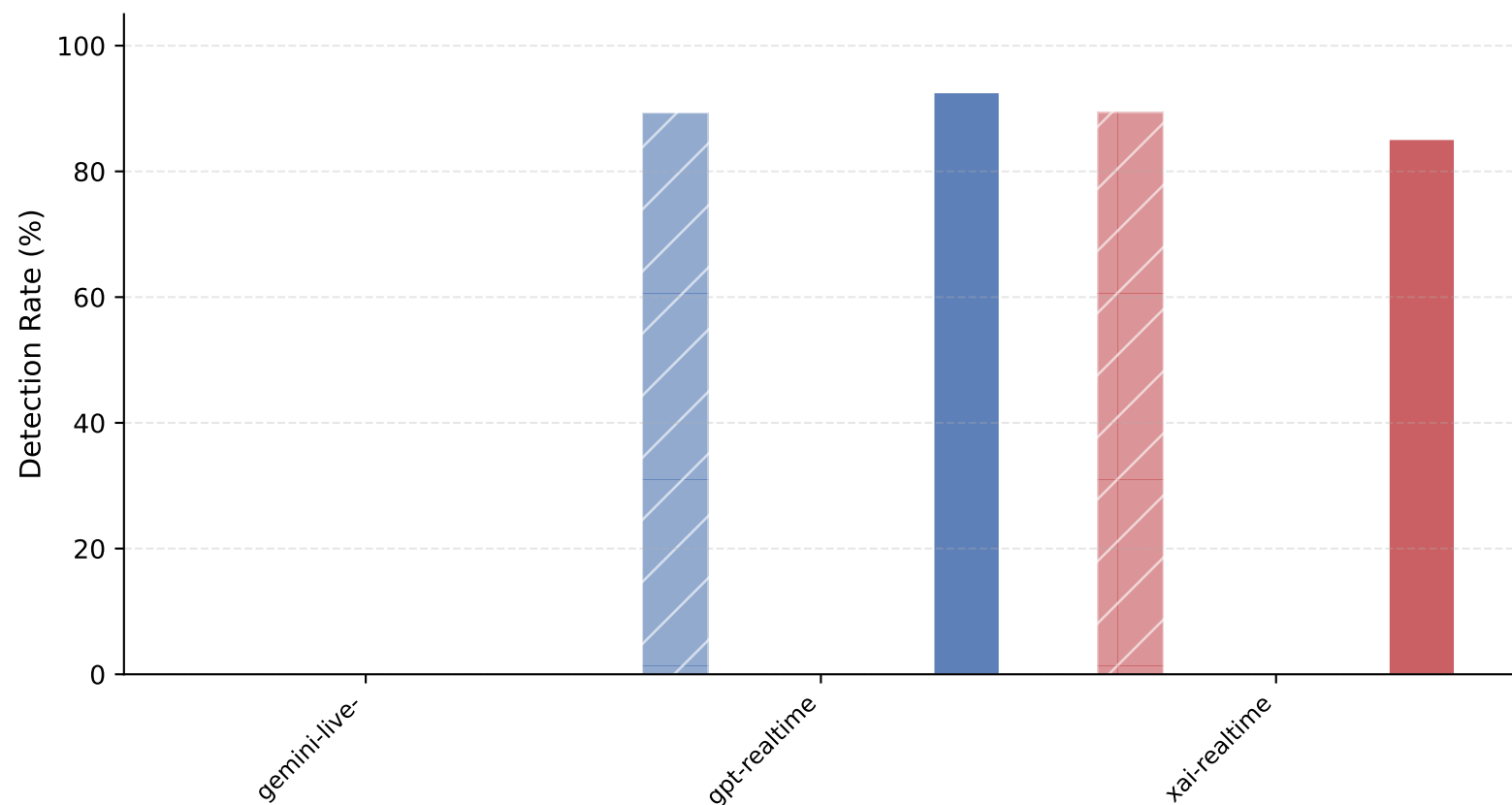
LLM Retail
