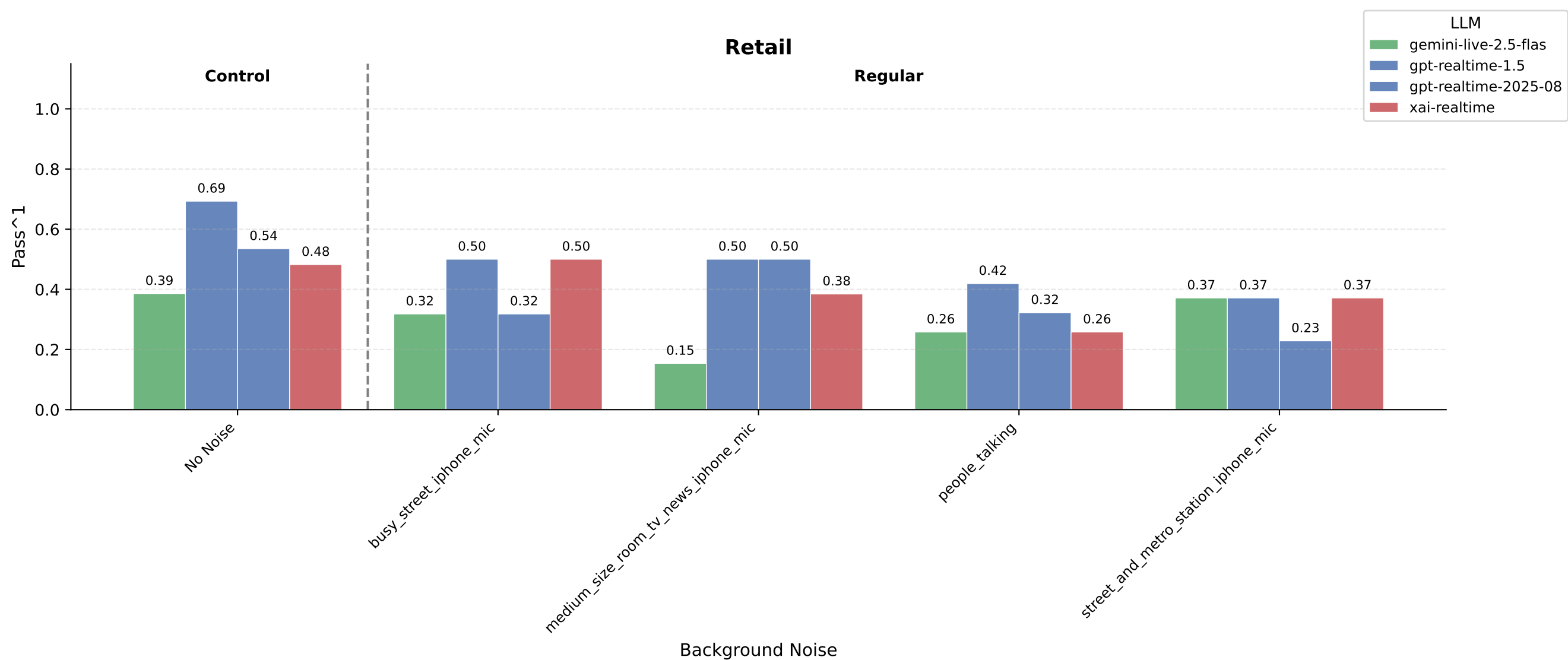
Pass^1 by Background Noise
