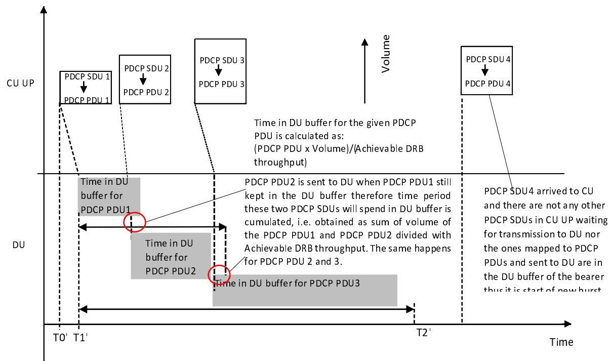
Figure 5.1.1.3.7-1 Average DL buffered UE throughput per DRB (SA, NSA option 3a)
