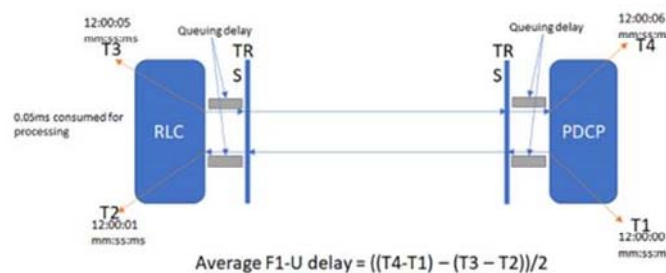
Figure 5.1.3.3.2-1 Average delay DL on F1U
