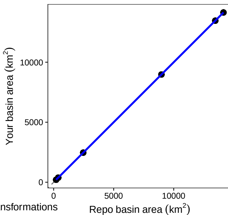
Sample-level basin area
