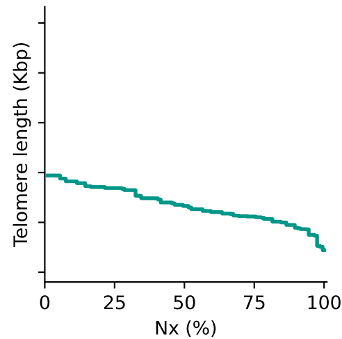
Crocodilians (n=2)
