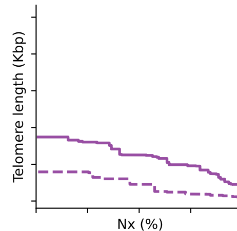
Amphibians (n=26)
