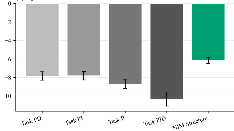
(c) Control Energy \downarrow
