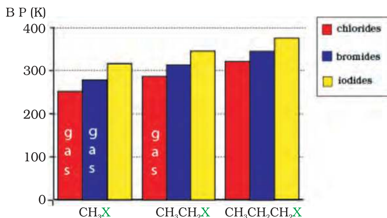
Fig. 6.1: Comparison of boiling points of some alkyl halides
