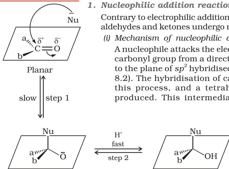
Fig.8.2: Nucleophilic attack on carbonyl carbon
