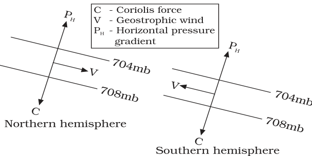
Figure 9.4 : Geostrophic Wind
