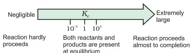
Fig. 6.6 Dependence of extent of reaction on K_c
