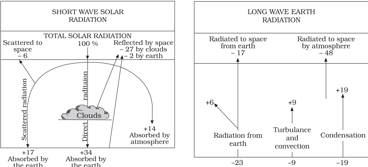
Figure 8.2 : Heat budget of the earth
