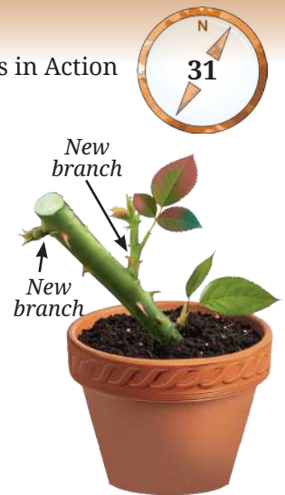
Fig. 3.5: New branches arising from the node of a stem
