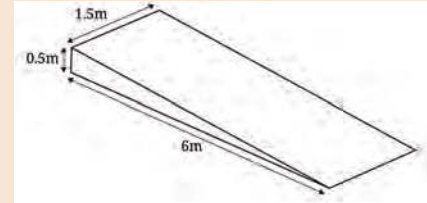
Figure 6.10: Drawing of a ramp with dimensions
